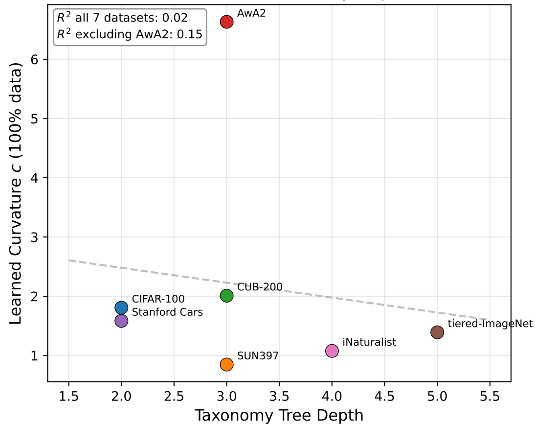
Curvature vs. Hierarchy Depth
