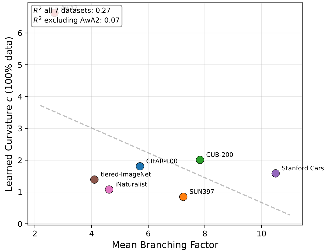
Curvature vs. Branching Factor
