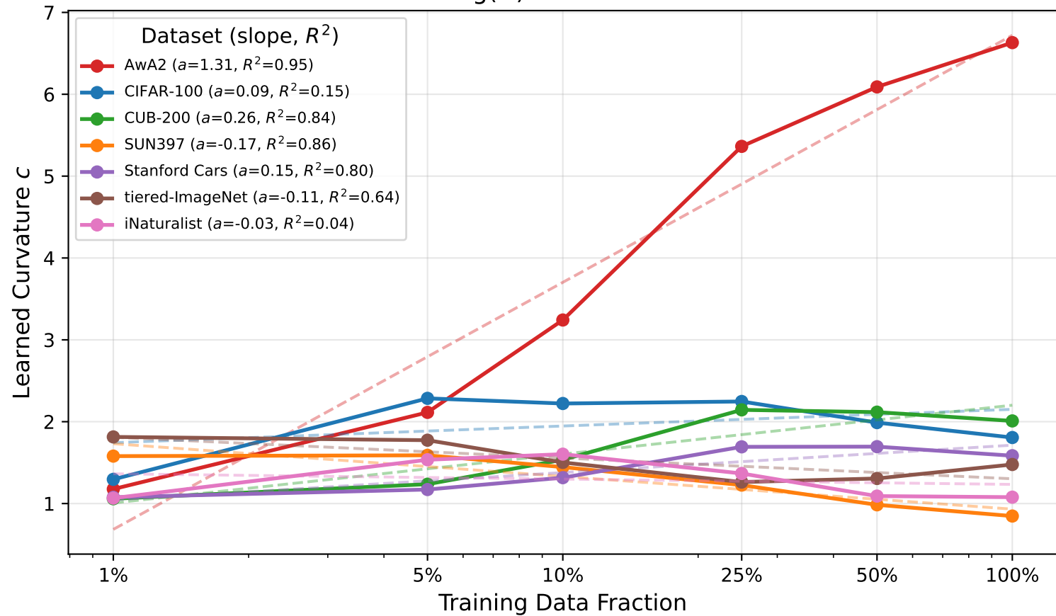
c \propto \log(N) Fit Per Dataset
