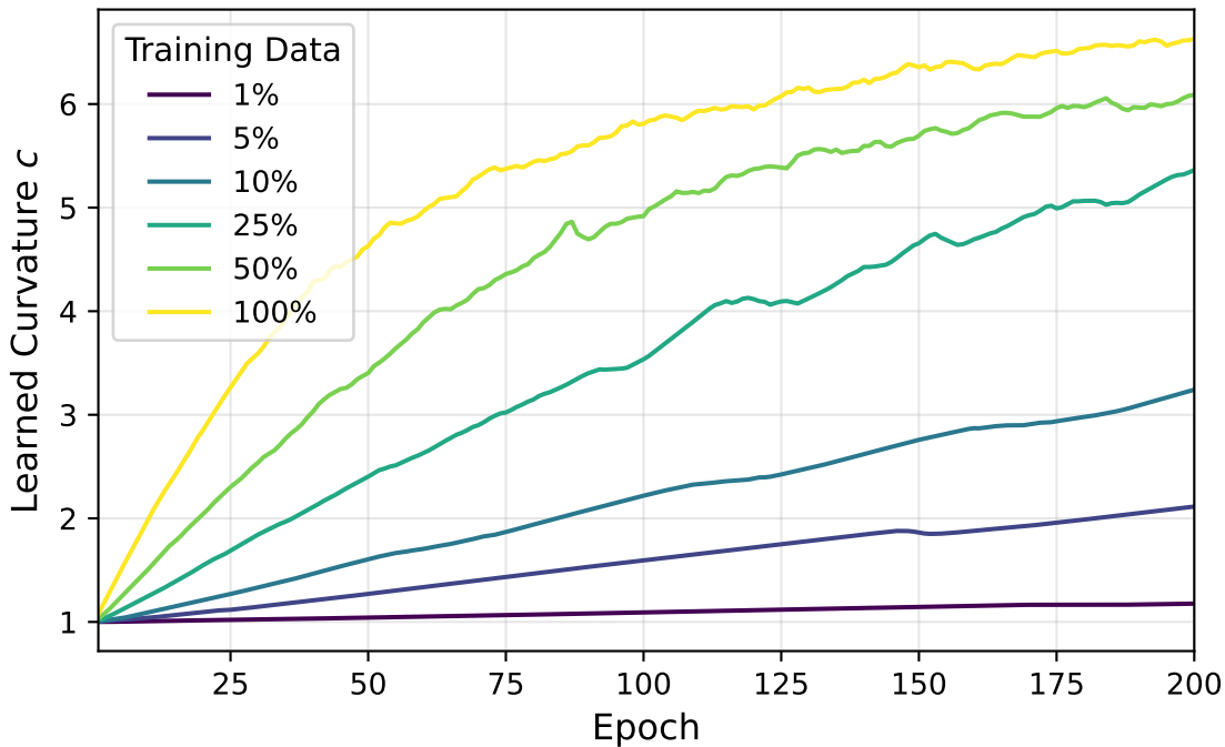
Poincaré Ball Curvature Evolution
