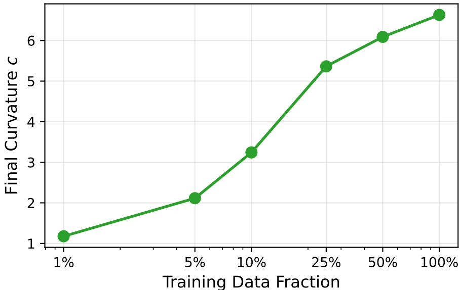
Learned Curvature Scales with Data Availability
