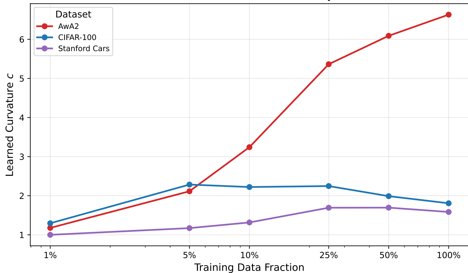
Learned Curvature Scales with Data Availability Across Datasets
