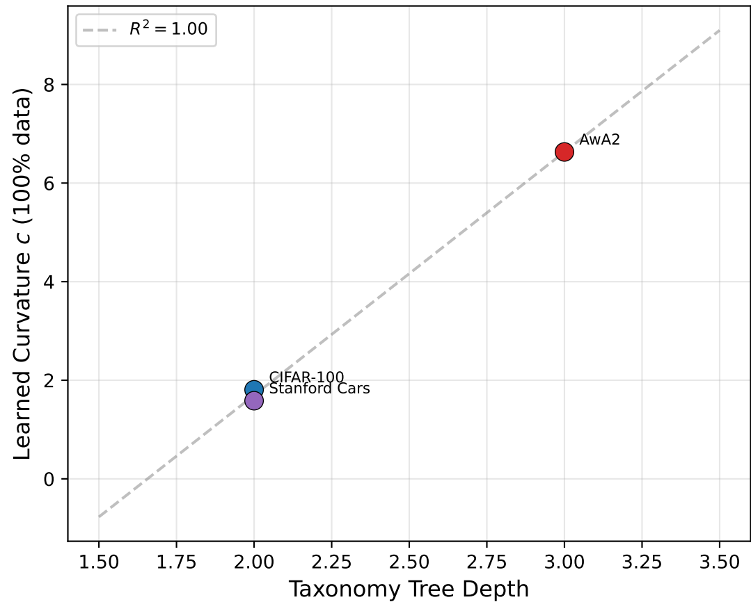
Curvature vs. Hierarchy Depth
