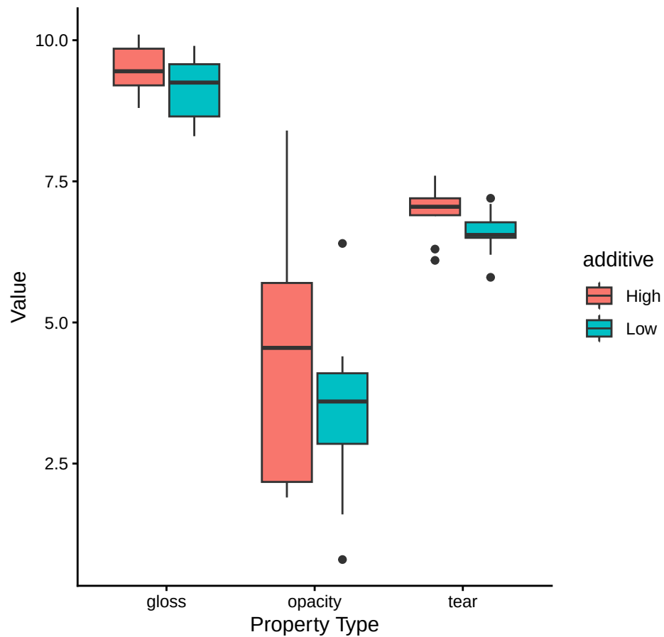
Plastic Properties by Additive Level
