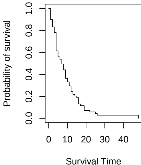
Kaplan-Meier Curve
