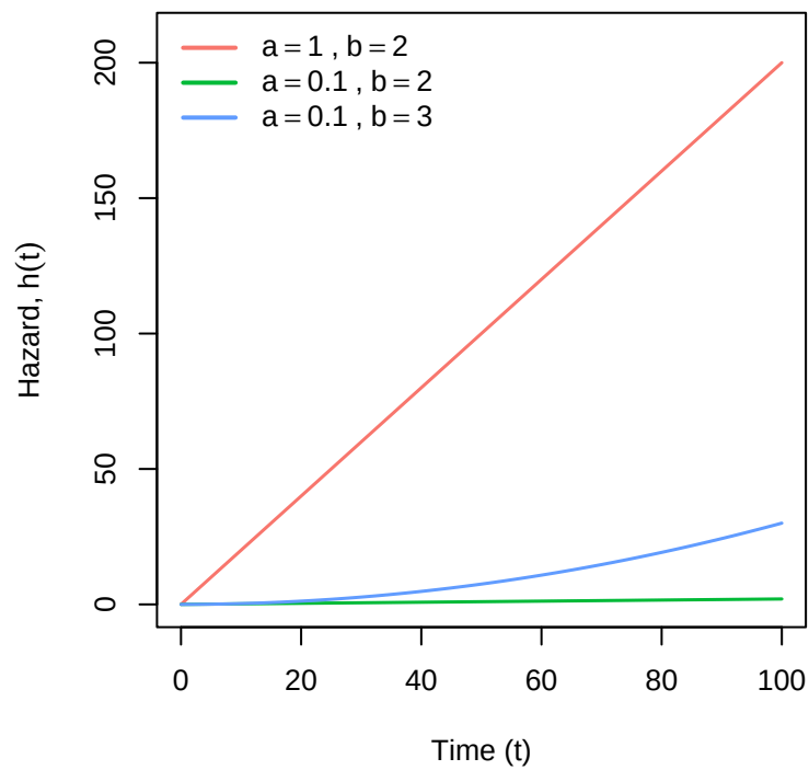
Log-Logistic
