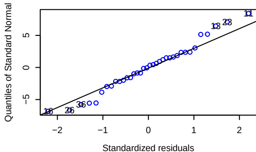
Normal Plot for Residuals
