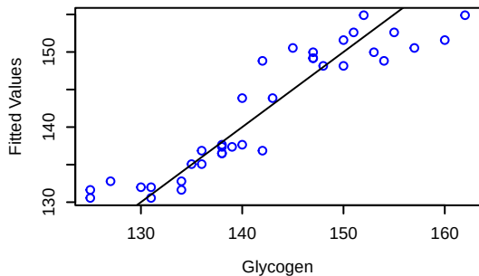
Fitted vs Observed
