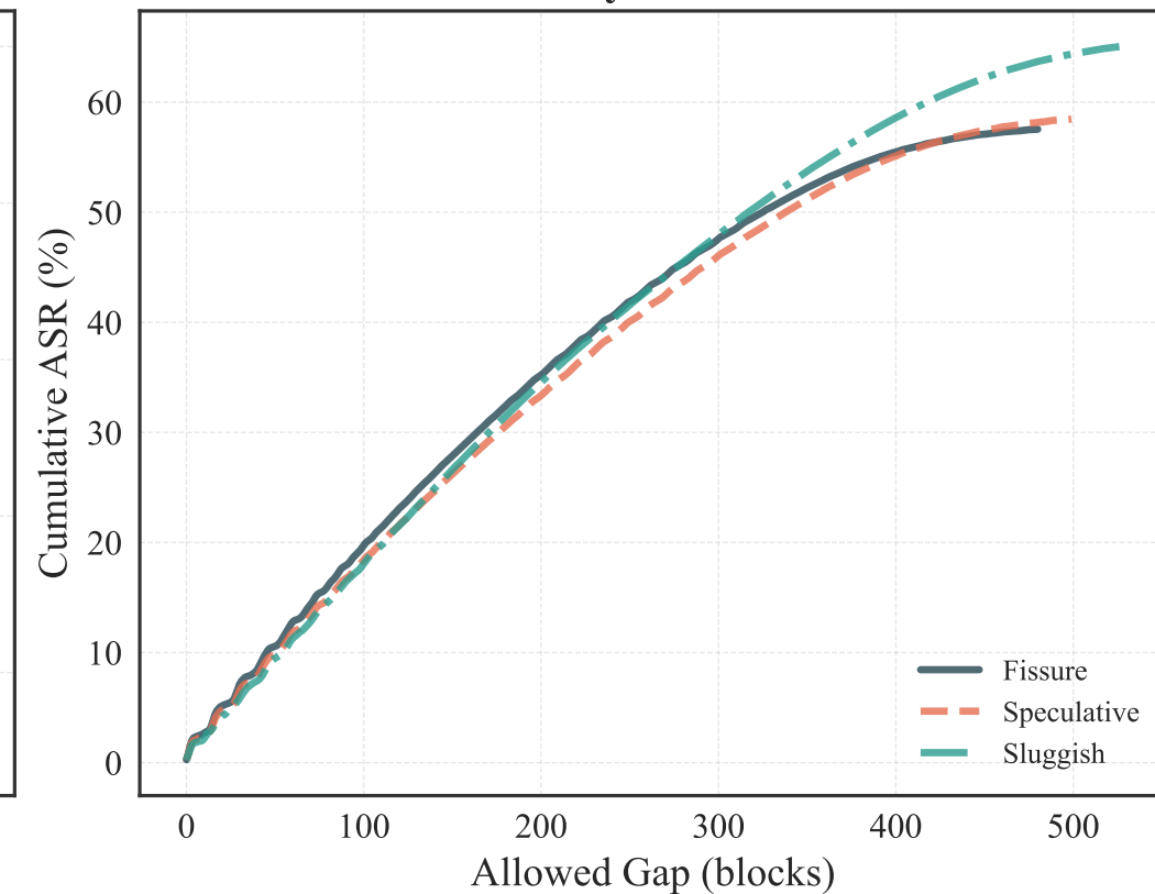
Mysticeti
