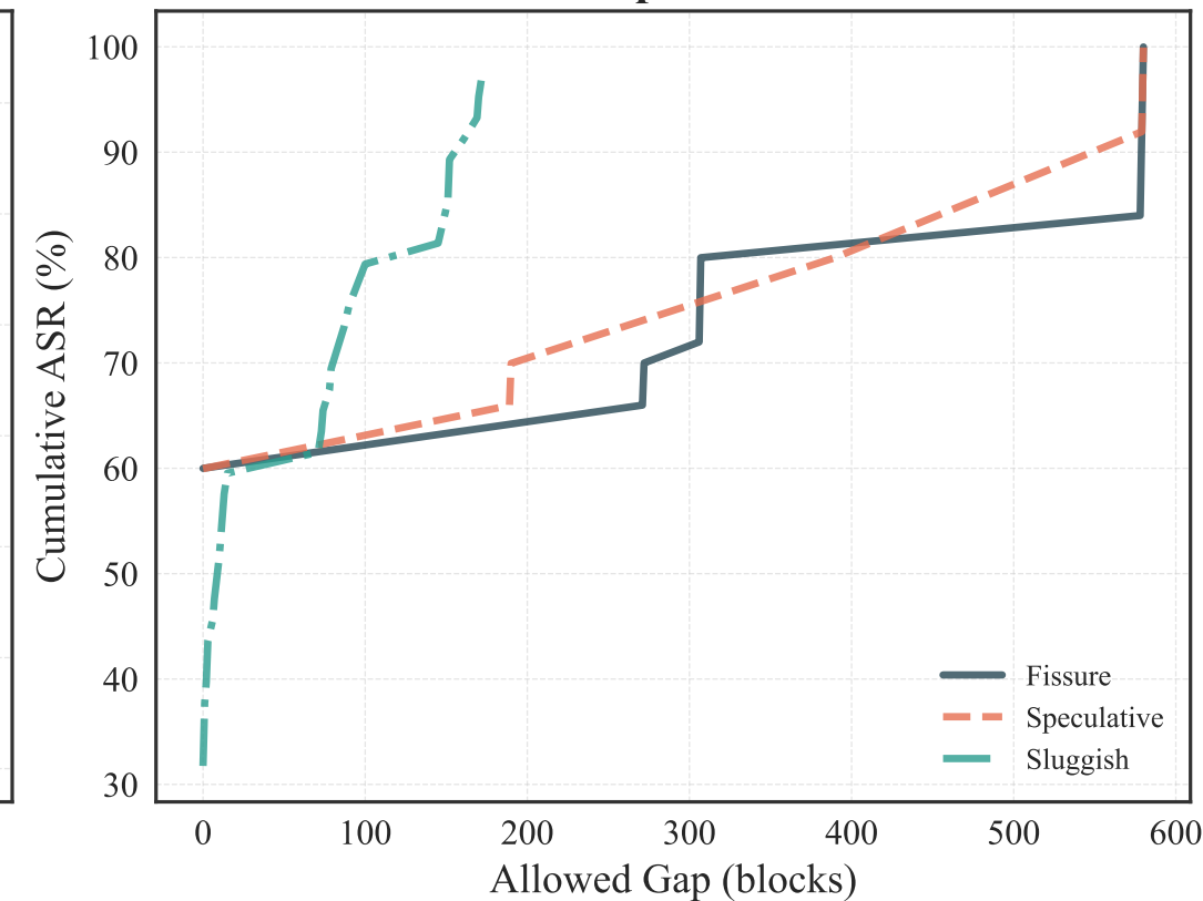
AlephBFT
