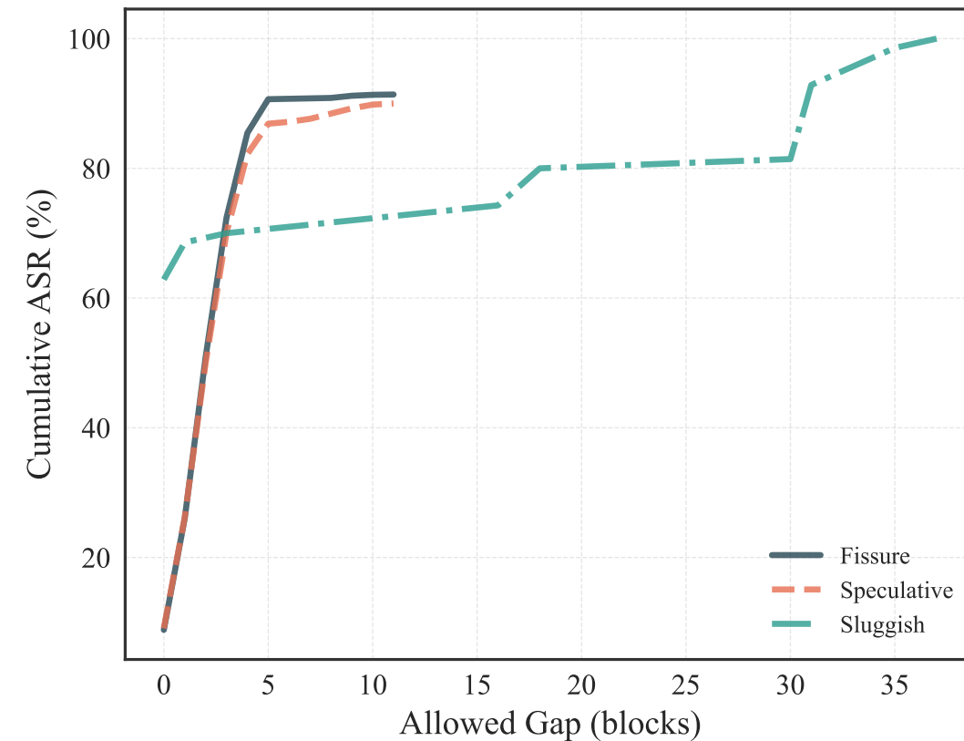
Bullshark
