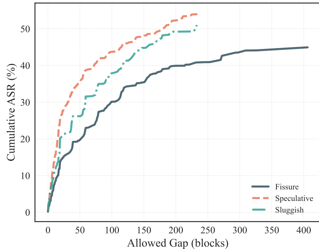
Autobahn
