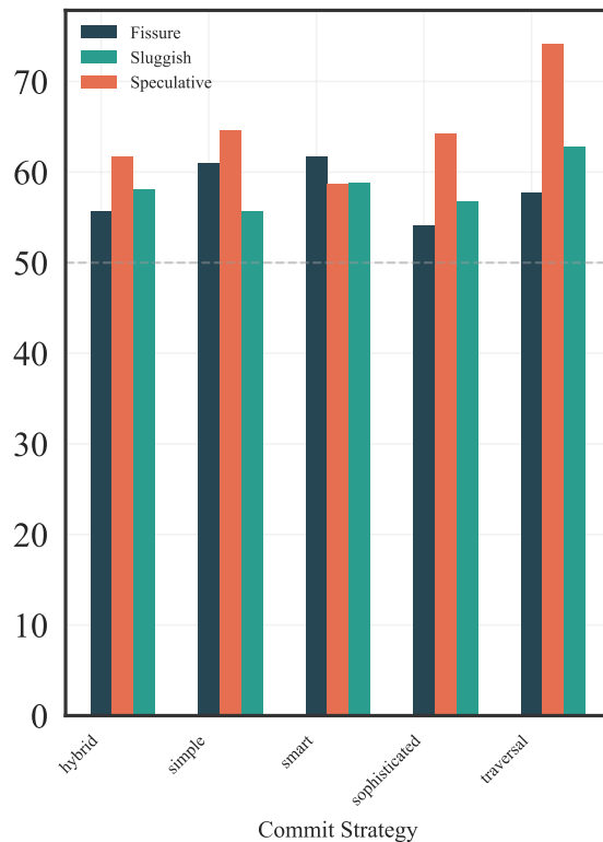
Protocol-Specific Parameters: Mahi Mahi / Mysticeti
