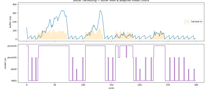
Figure 6: Energy-harvesting scenario. The adaptive policy tracks the buffer level—running costlier models at peaks, cheaper ones during lulls—yet does not exceed a well-chosen static policy, because the 50%-pruned model is sustainable on the mean harvested power.
