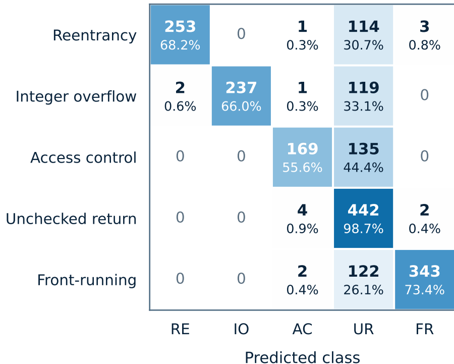
(a) Five-class GNNMHA v2 ( n = 1,949 )
