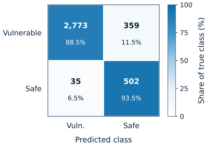
(b) Stage-A binary gate ( n = 3,669 )
