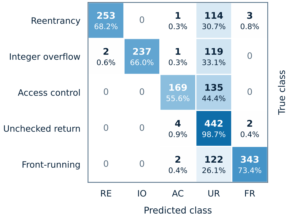
(a) Five-class GNNMHA v2 ( n = 1,949 )
