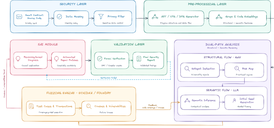
Fig. 1. PRISM architecture: PrivacyFilter and DataMasker scrub sensitive tokens, the contract is parsed to a CPG, screened by the Stage-A binary gate and GNNMHAv2 five-class ranker, and prioritized functions are passed to a local LLM to generate Foundry fuzzing harnesses with concrete EVM execution.
