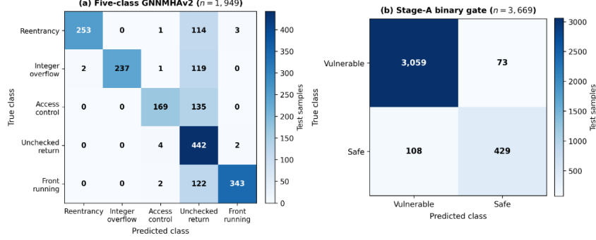
Fig. 2. (a) Five-class confusion matrix of GNNMHA v2 on the random-split test set (RE: reentrancy, IO: integer overflow, AC: access control, UR: unchecked return, FR: front-running). (b) Stage-A binary gate.
