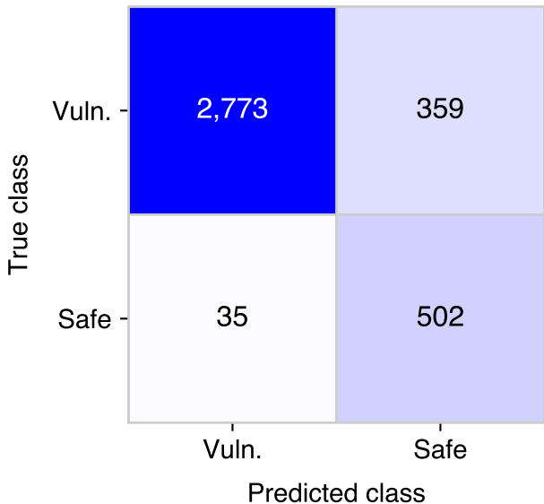
(b) Stage-A binary gate ( n = 3,669 )
