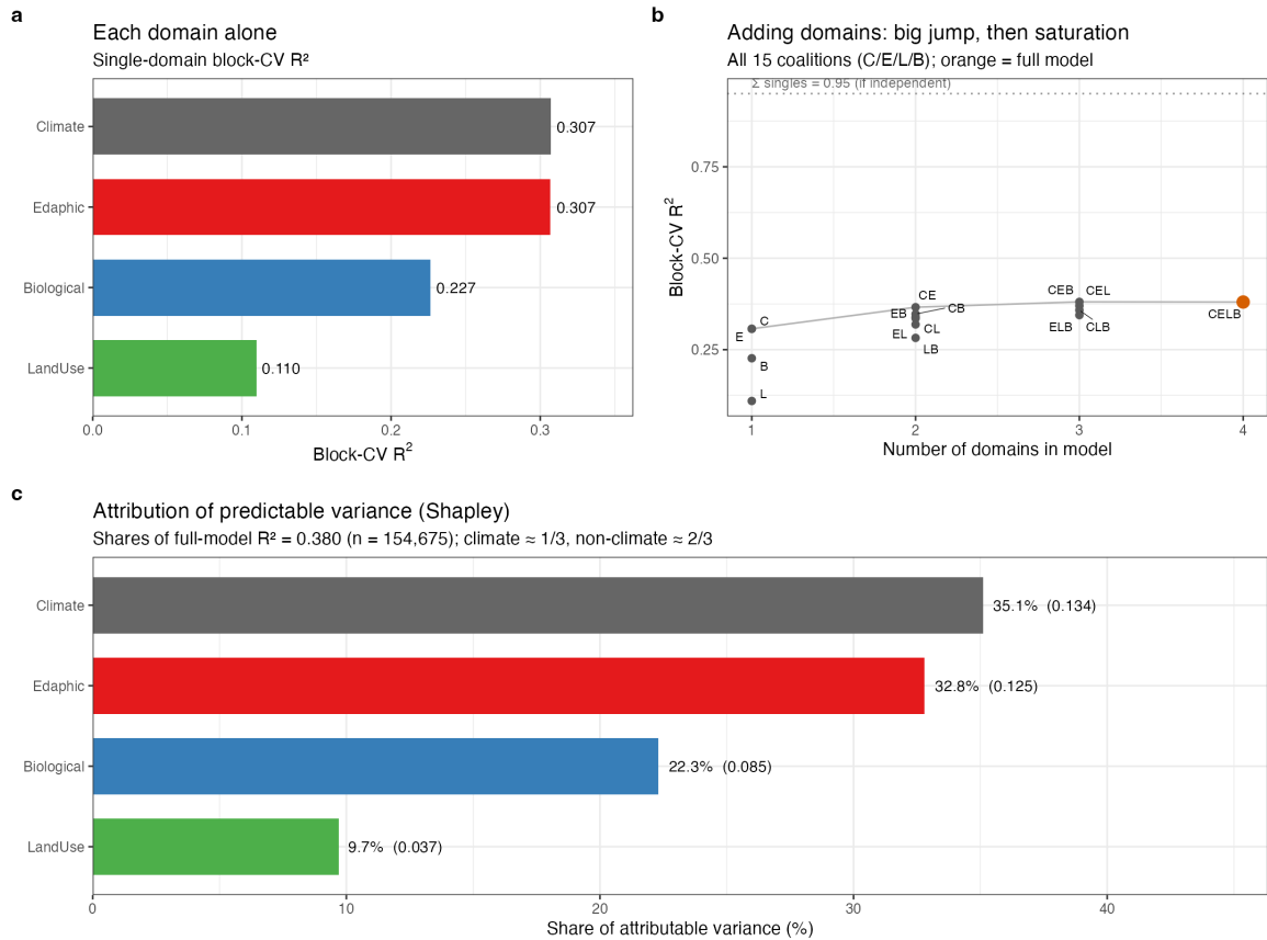
Spatially-honest variance decomposition of soil-carbon turnover
