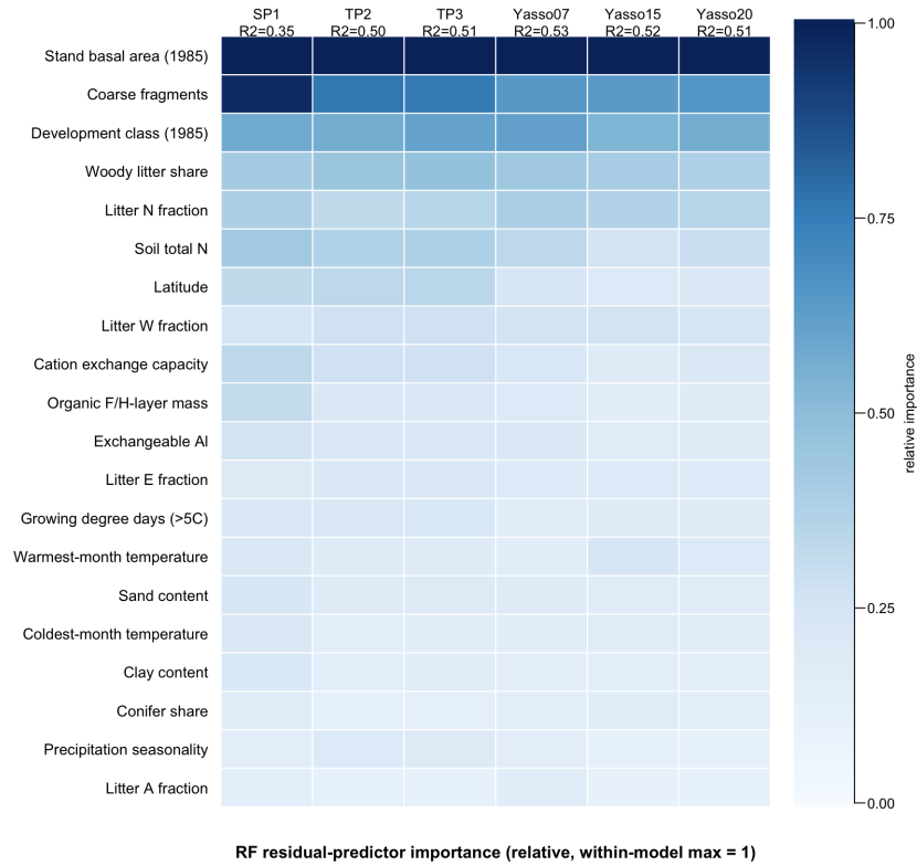
Figure 11: Residual structure. Random-forest importance of candidate drivers for the plot-level residuals (relative, within model). Stand basal area leads in every model; the residual points to site productivity and inputs, not to kinetics.
