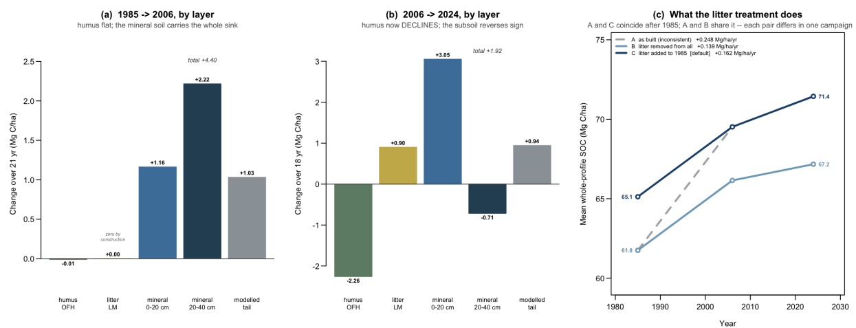
Figure 22: S9 — where the apparent SOC change sits, by layer. (a,b) change per layer over each inter-campaign interval. The humus layer is flat over 1985–2006 (–0.01) and declines over 2006–2024 (–2.26), while the mineral soil carries the entire apparent sink and the subsoil reverses sign (+2.22 then –0.71). A genuine accumulation signal should be surface-weighted; this one is depth-weighted. (c) the litter treatment as a bracket on the observed trend: A as built (1985 without LM, 2006/24 with — internally inconsistent), B litter removed from all three, C litter added to 1985 (working default). Panels (a,b) are on basis C, under which the 1985–2006 LM bar is zero by construction and is drawn hollow to say so. Conditional on the 1985 record being OFH-only (see text).
