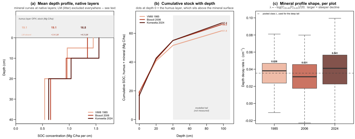
Figure 21: S8 — SOC depth distribution of the three campaigns. All panels on one basis: humus (OFH) + mineral, with the litter layer (LM) excluded because it is absent from the 1985 record; its size is printed in (a). (a) mean profile at each campaign's native layers (VMI8 splits 0–20 as 0–5/5–20, the later campaigns as 0–10/10–20). (b) cumulative stock with depth, the sub-40 cm tail shaded as modelled, not measured. (c) the interval-free shape statistic \lambda = -\log(C_{20-40}/C_{0-20})/20 , medians 0.038 / 0.031 / 0.041 \text{cm}^{-1} . 1985 sits between the other two , so the profile shape does not single it out — the campaign difference is a level, not a distortion of the depth distribution.
