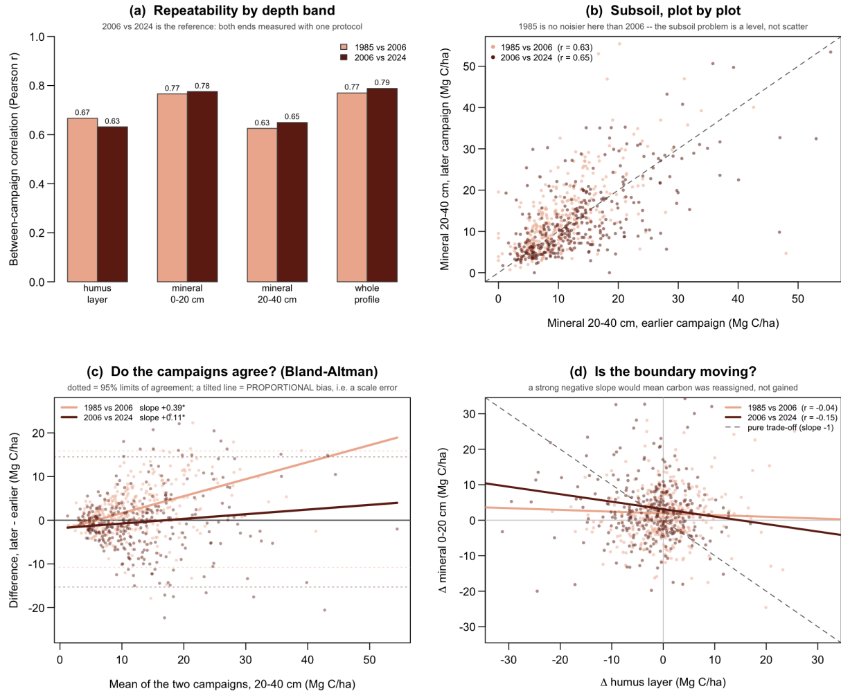
Figure 23: S10 — campaign repeatability, agreement, and the organic/mineral boundary. (a) between-campaign correlation by layer; 2006 vs 2024 is the reference pair, both ends measured under one protocol. (b) the subsoil plot by plot: 1985 is no noisier than 2006 ( r = 0.63 vs 0.65 ), so the subsoil problem is a level offset, not scatter. (c) Bland–Altman agreement for the subsoil — the difference between campaigns against their average (neither is a gold standard). A non-zero intercept is a constant bias; a tilted line is proportional bias, the fingerprint of a scale error (bulk density, sampled volume) rather than an added amount of carbon. 1985–2006 slope +0.39 , equivalent to C_{2006} \approx 1.48 C_{1985} - 2.8 . Note the limits of agreement, -10.8 to +15.9 \text{ Mg C ha}^{-1} on a layer holding \sim 11 : the mineral data cannot resolve plot-level change in either pair. Proportional bias is present in every campaign pair and both mineral layers (0–20 cm: +0.17 for 1985–2006, +0.34 for 2006–2024), so it is a property of the mineral measurement in general, not of 1985 alone. (d) the boundary test — the organic/mineral split is set by eye in the field, so carbon can be reassigned between the humus and mineral 0–20 cm bands with no carbon moving; a pure reassignment would follow the dashed slope -1 . Observed r = -0.04 (1985–2006) and -0.15 (2006–2024): a weak effect in the later pair only.
