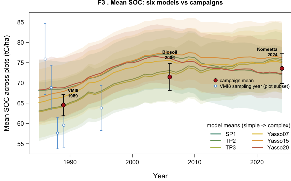
Figure 4: The central result. Cross-plot mean SOC, all six models, 1985–2024: rise then bend toward saturation, tracking the Biosoil/Komeetta campaign means. Colour runs from the simple models (green) to the Yasso family (warm).
