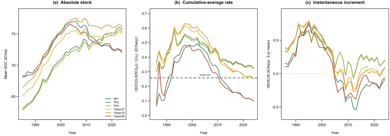
Figure 1: The same six calibrated trajectories under three transforms. (a) absolute mean SOC; (b) the cumulative-average rate (SOC(t) - SOC(t_0))/(t - t_0) used in the earlier increment figure; (c) the instantaneous annual increment (5-year mean). The decline in (b) is the deceleration of a still-rising stock, not a loss of carbon.
