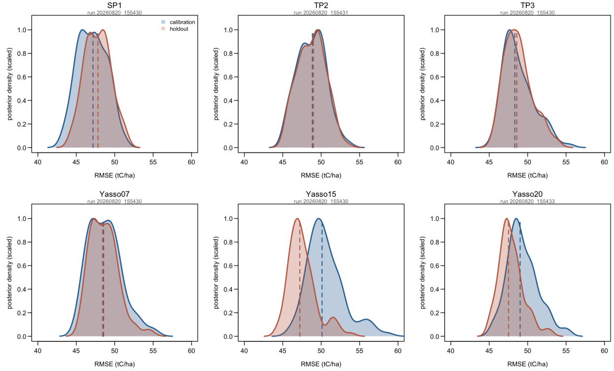
Figure 2: Posterior distribution of RMSE, one panel per model, recomputed for each of the 100 posterior draws. Blue = calibration plots, red = held-out plots; dashed lines are medians; densities are scaled to a common height so shape is comparable across panels. The horizontal range is held fixed across runs so that successive calibrations can be laid side by side.
