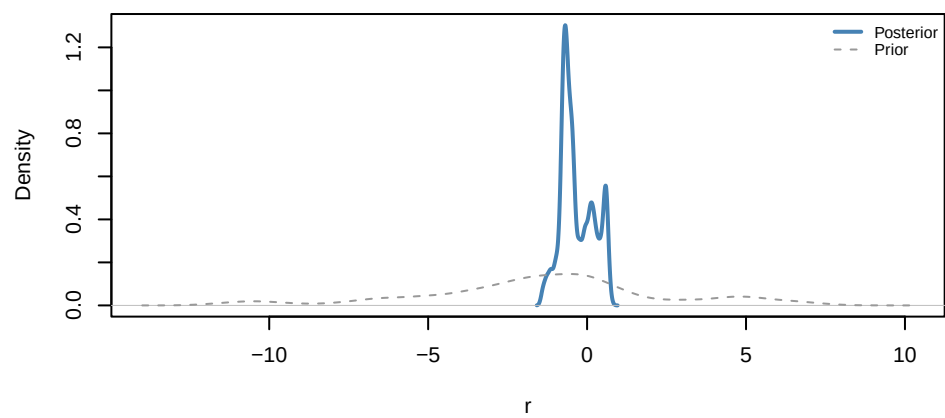
Yasso07 | sigma_init
