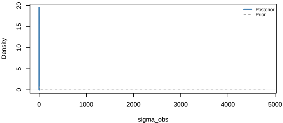
Yasso07 | sigma_obs
