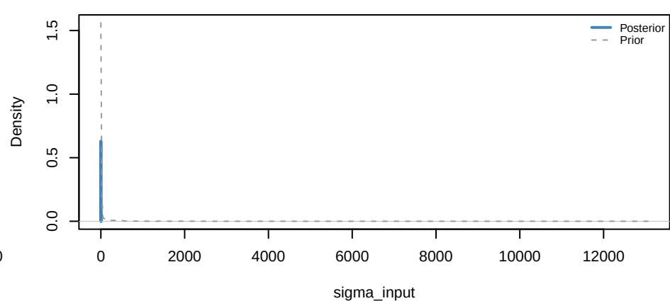
Yasso07 | sigma_input
