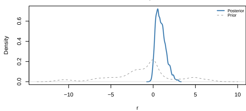
Yasso07 | sigma_input
