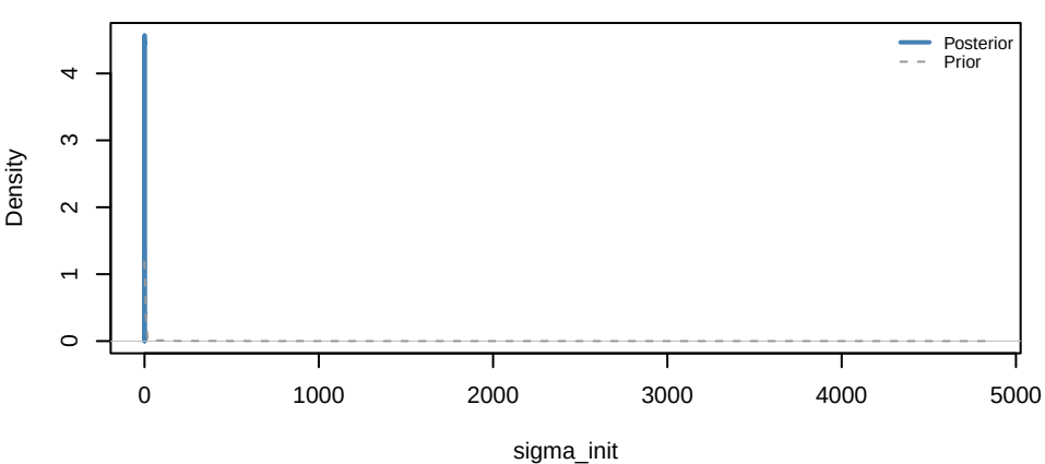
Yasso07 | sigma_init
