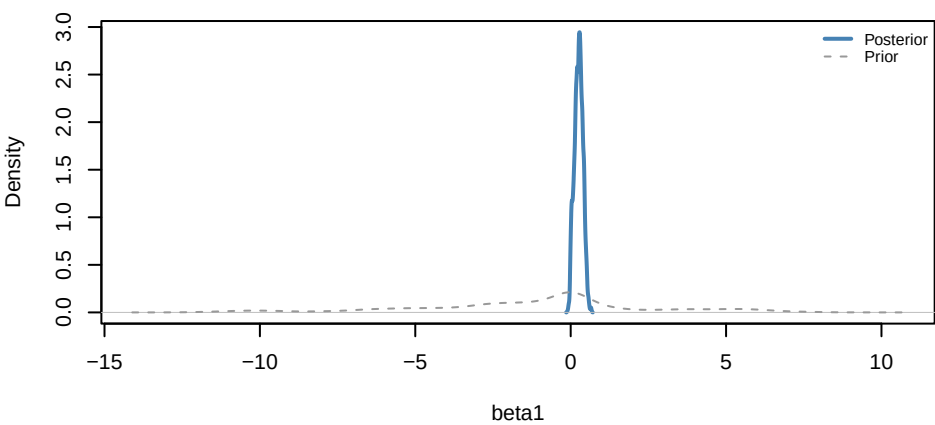
Yasso07 | gamma
