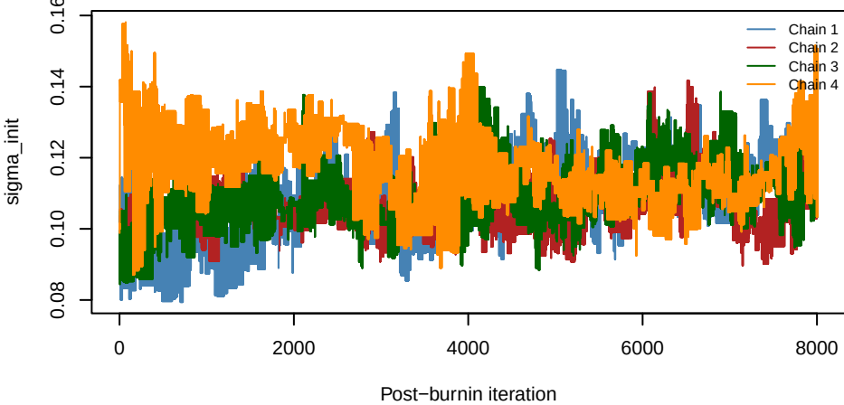
Yasso07 | sigma_init | 20260217_150338
