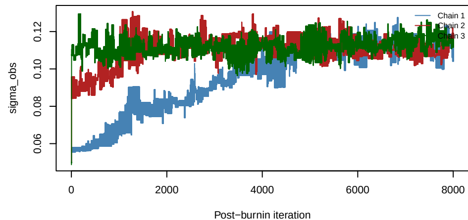
Yasso07 | sigma_obs | 20260220_093211
