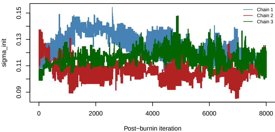
Yasso07 | sigma_init | 20260220_093211
