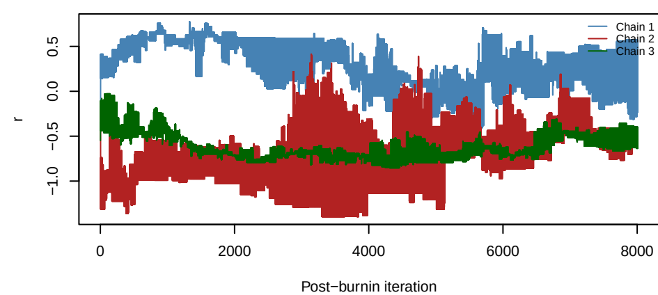
Yasso07 | sigma_init
