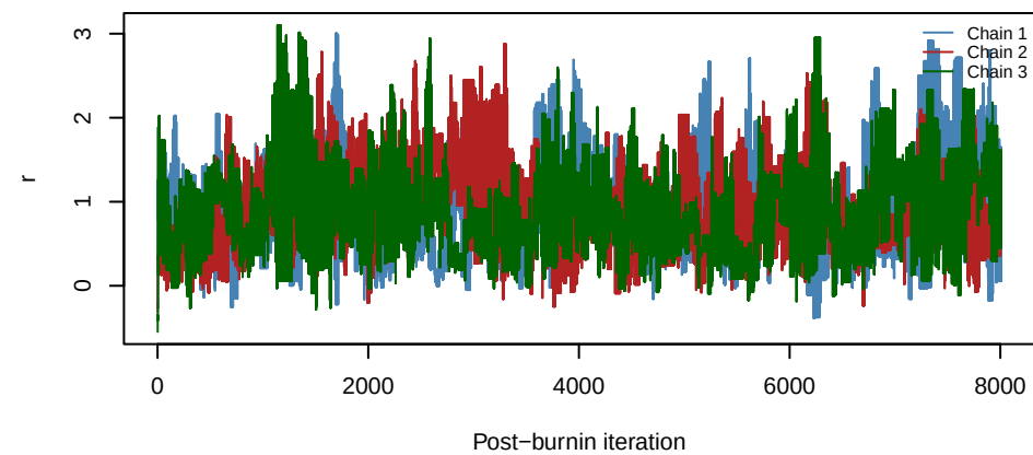
Yasso07 | sigma_input
