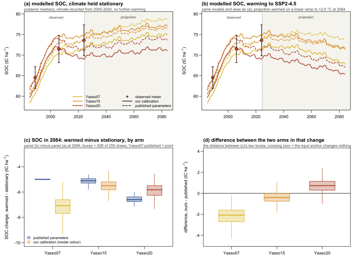
Figure 9: Projections from the published parameterisation and from the calibration, under the same scenarios. Neither arm was recalibrated, and only the litter input multiplier was refitted, so that both arms reproduce the observed window equally well and any later divergence is extrapolation rather than fit. Only Yasso07 separates the two arms.
