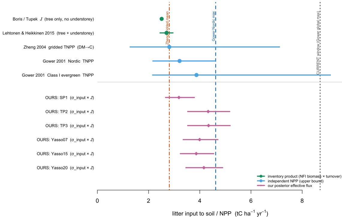
Figure 8: The litter input inferred by the calibration, against independent estimates of the same flux. Green symbols are inventory-based litter products, blue symbols are independent estimates of net primary production, which bound the litter flux from above, and the lower group shows the effective flux inferred here for each of the six models. Bars are reported ranges for the literature estimates and 95% posterior intervals for the models.
