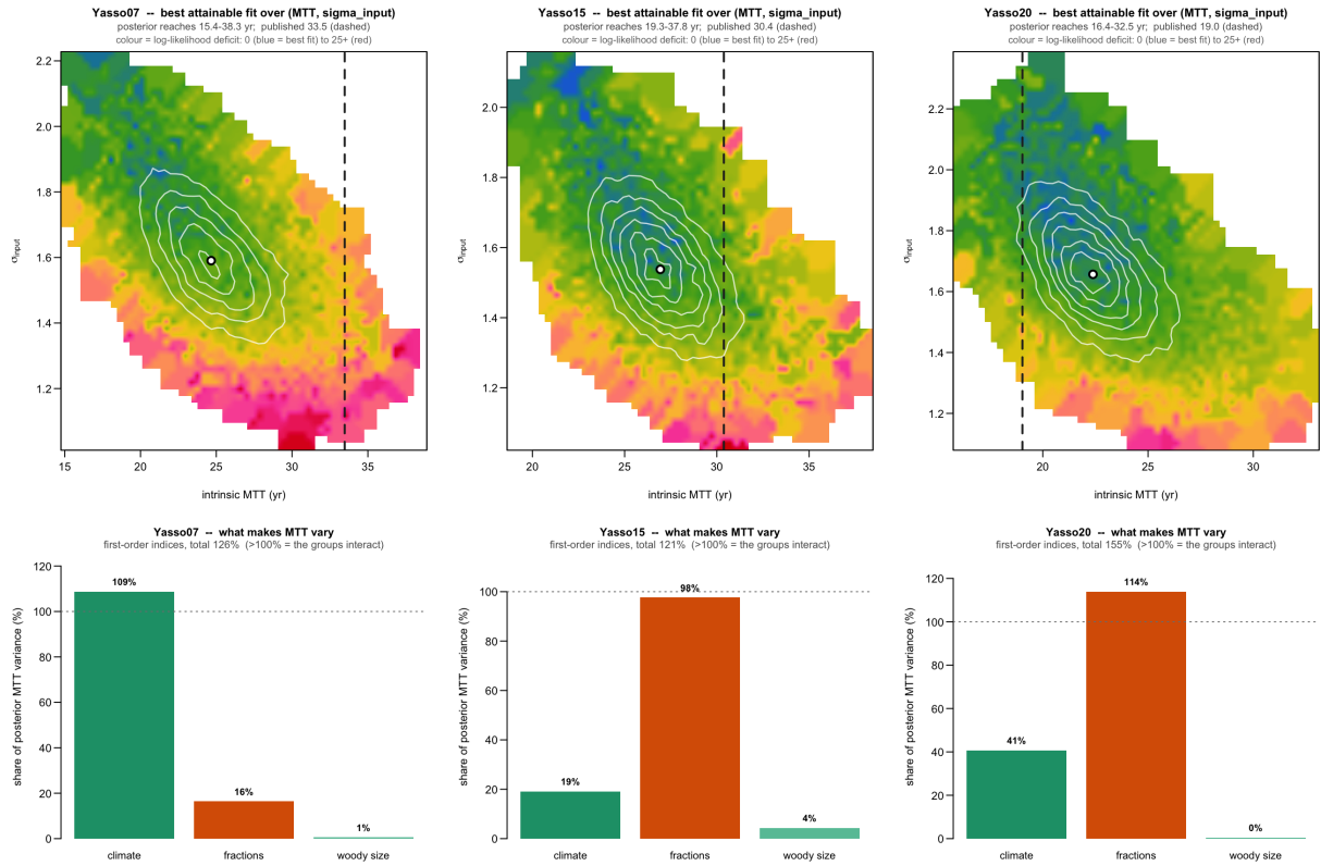
Figure 7: The trade-off between transit time and litter input. For each version of Yasso, the best fit to the data attainable at each combination of mean transit time and litter input multiplier. The colours show the fit to the data alone, with the priors excluded , from blue at the best fit through green and yellow to red at the worst. The white contour lines show the posterior, which combines the fit to the data with the priors. The dashed line marks the published transit time and the white dot marks the posterior median. Cells that the sampler visited fewer than five times are left blank, and a blank cell means that the region was not visited rather than that the region cannot be fitted. The offset between the bluest colour and the innermost contour measures how far the priors pull the answer away from where the data alone would place it.
