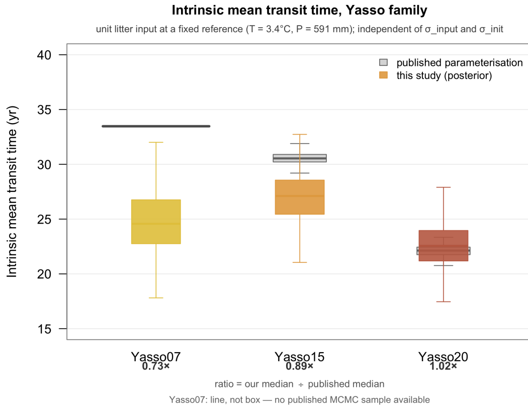
Figure 6: Mean transit time of carbon in the three versions of Yasso, calibrated and published. Transit times are computed at a common reference climate and litter composition, from the model equations alone, so that the comparison depends neither on the litter input multiplier nor on the starting state.
