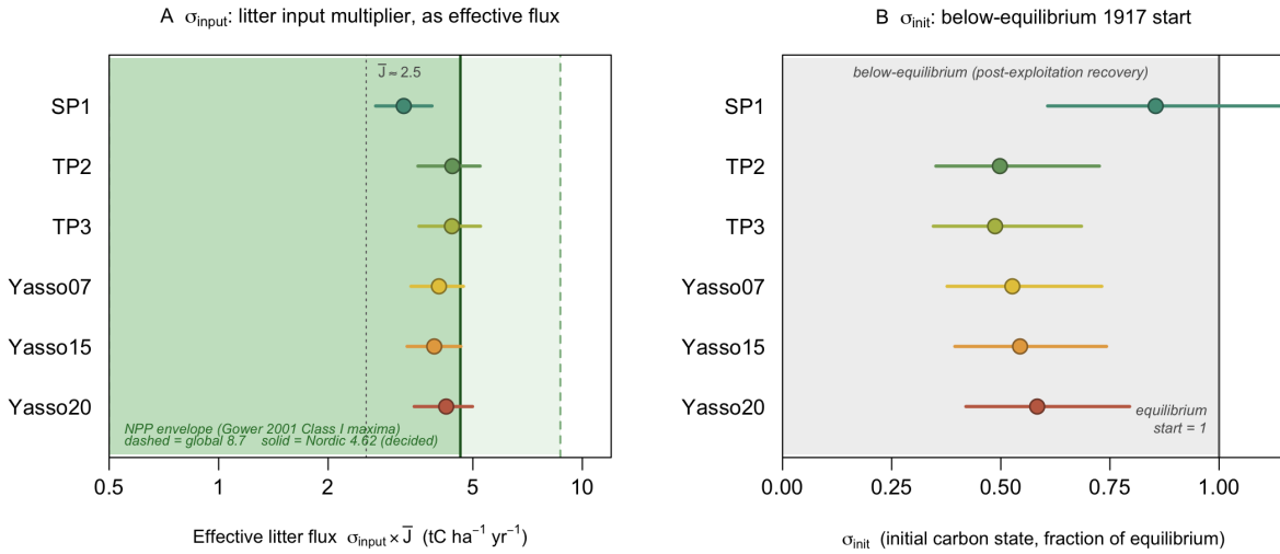
Figure 5: The two estimated auxiliary quantities, read as physical quantities. Left: the litter input multiplier expressed as an effective flux of litter carbon to the soil, that is, the multiplier times the litter input that the product supplies. The dotted line marks the flux the product itself supplies, and the shaded bands mark the envelope of independent estimates of boreal net primary production. Every model settles above the tree litter the product supplies and inside the envelope. Right: the estimated ratio of the 1917 litter input to the 1985 litter input. All six models place the 1917 input below the 1985 input, which is the direction the forest history requires.
