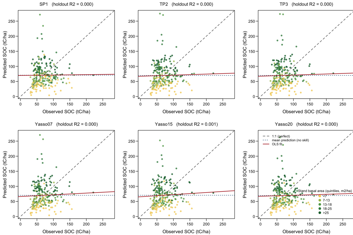
Figure 10: Predicted against measured soil carbon on held-out plots. Points are coloured by the standing basal area of the plot, in quintiles. The dashed line is the one-to-one line, the dotted line is the prediction of the mean, and the solid line is the fitted relation. The predicted stocks spread more widely than the measured stocks and are ordered by basal area, whereas the measured stocks are not.
