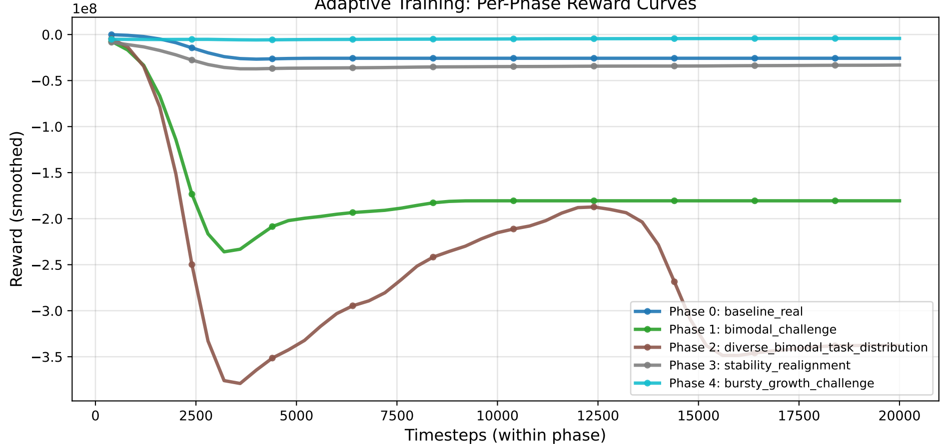
Adaptive Training: Per-Phase Reward Curves
