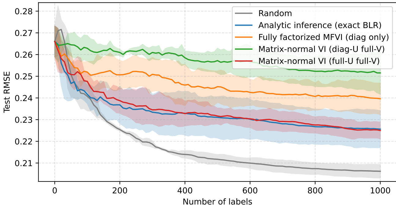
Regression AL: inference comparison
