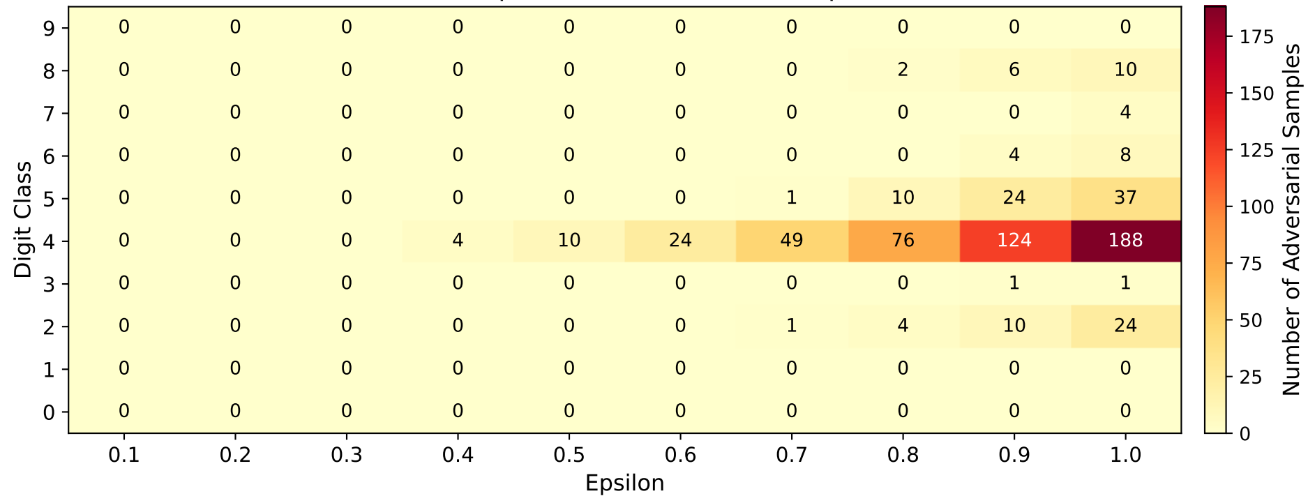
Adversarial samples across classes and Epsilon-ball
