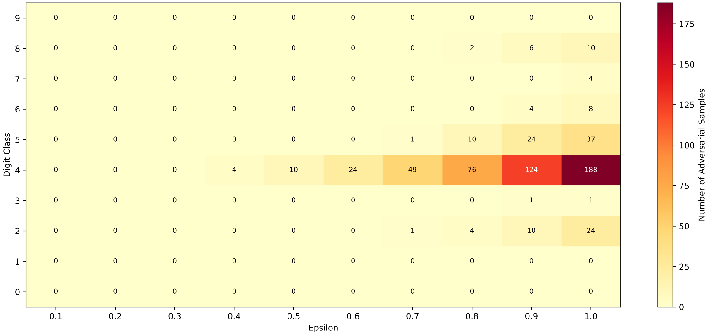
Adversarial Samples Across Classes and Epsilon-ball
