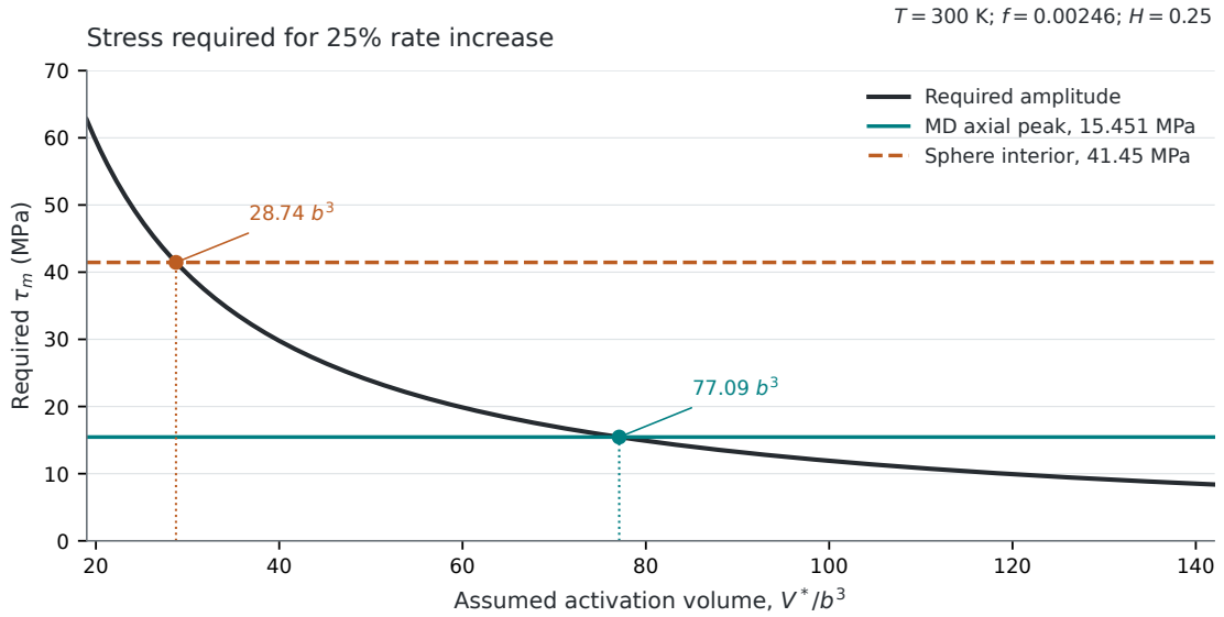
Both stress scales enter the same assumed r^{-3} distribution and two-scale integral. Activation volume and inclusion strain are conditional inputs to this comparison.
