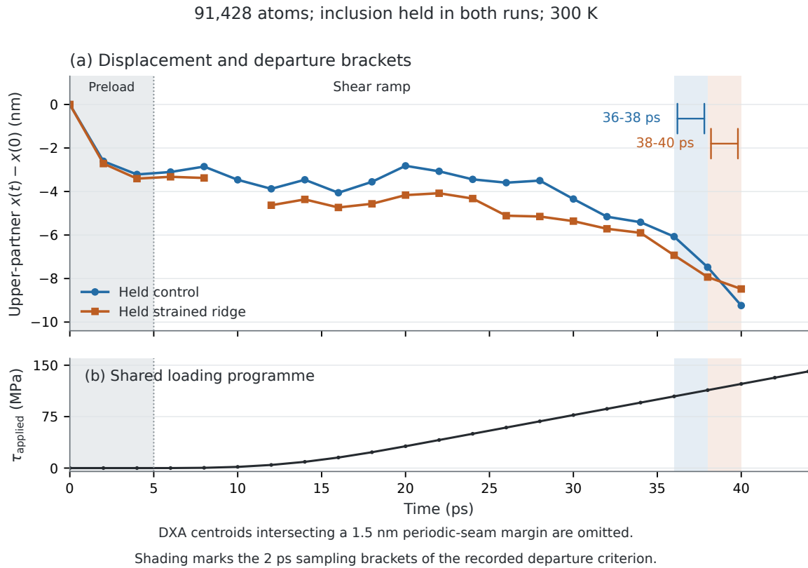
Figure 3: Existing-line motion in the interface cells. Upper-line positions are followed through preconditioning and shear loading, with the applied stress shown alongside. The restrained control and perturbed cases cross the departure criterion one saved frame apart. The initial motion towards the ridge and the retained DXA segments at the periodic seam constrain interpretation of the later trajectories. Segment disappearance or reassignment is not evidence of a new interface dislocation.
