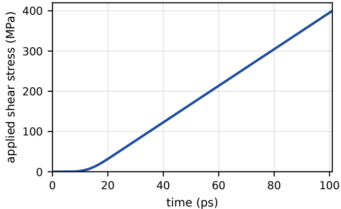
(a) interface cell with the dislocation pair: ramp to 400 MPa
