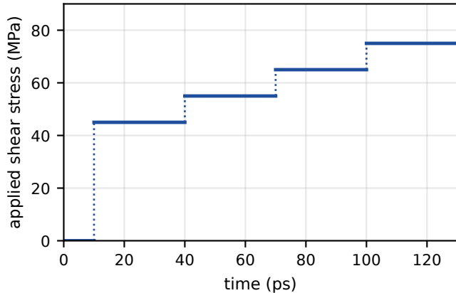
(b) alloy cell: constant-stress steps
