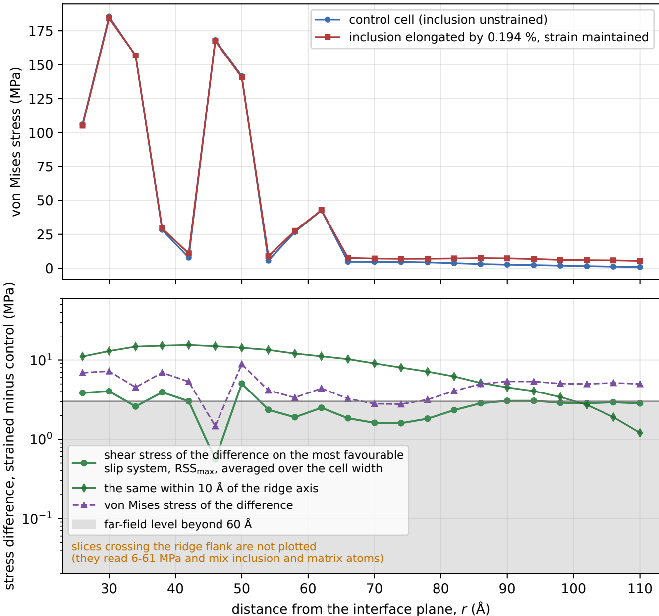
Stress in the Al matrix against the distance from the \text{Al}_{13}\text{Fe}_4 interface
