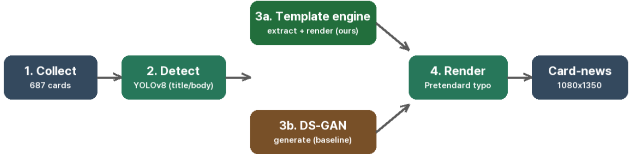
Figure 2. System overview. A shared detector feeds two generation routes; the template engine (3a) is our deployed path, DS-GAN (3b) is the research baseline.
