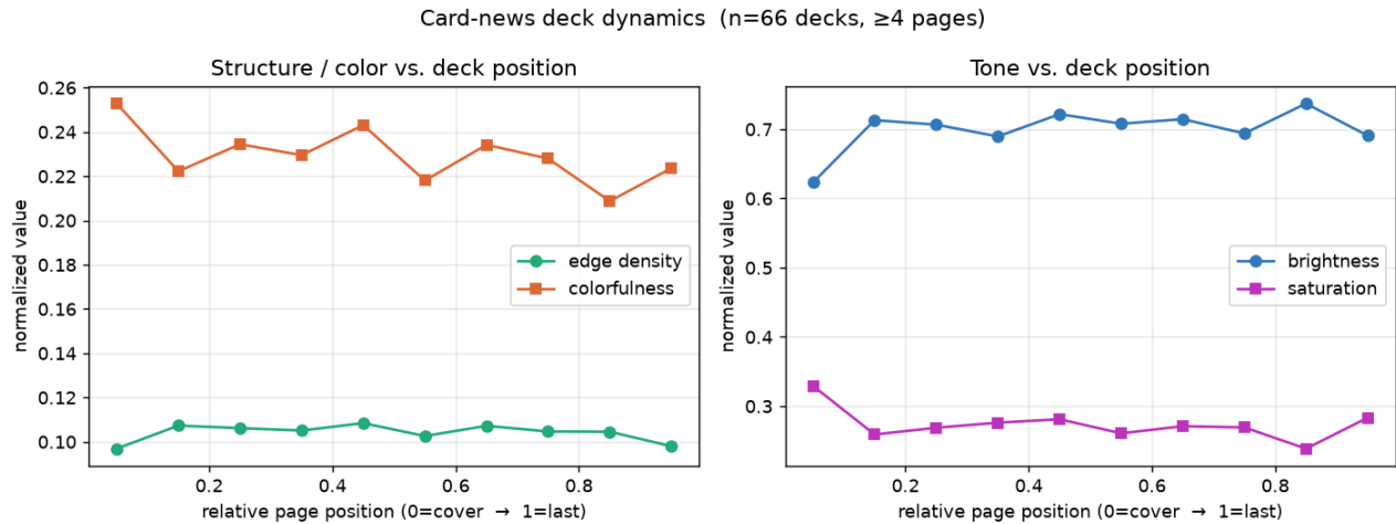
Figure 3. Deck dynamics across relative page position (66 decks). Covers are darker, more saturated/colorful and less edge-dense than interior pages.
