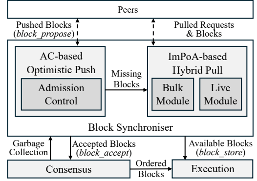
Figure 4: Beluga can be integrated into a generic BFT consensus protocol. By applying the consensus rules on the blocks produced by Beluga, validators derive a consistent order for blocks. Beluga guarantees the availability of ordered blocks for the state machine replication (SMR) execution.
