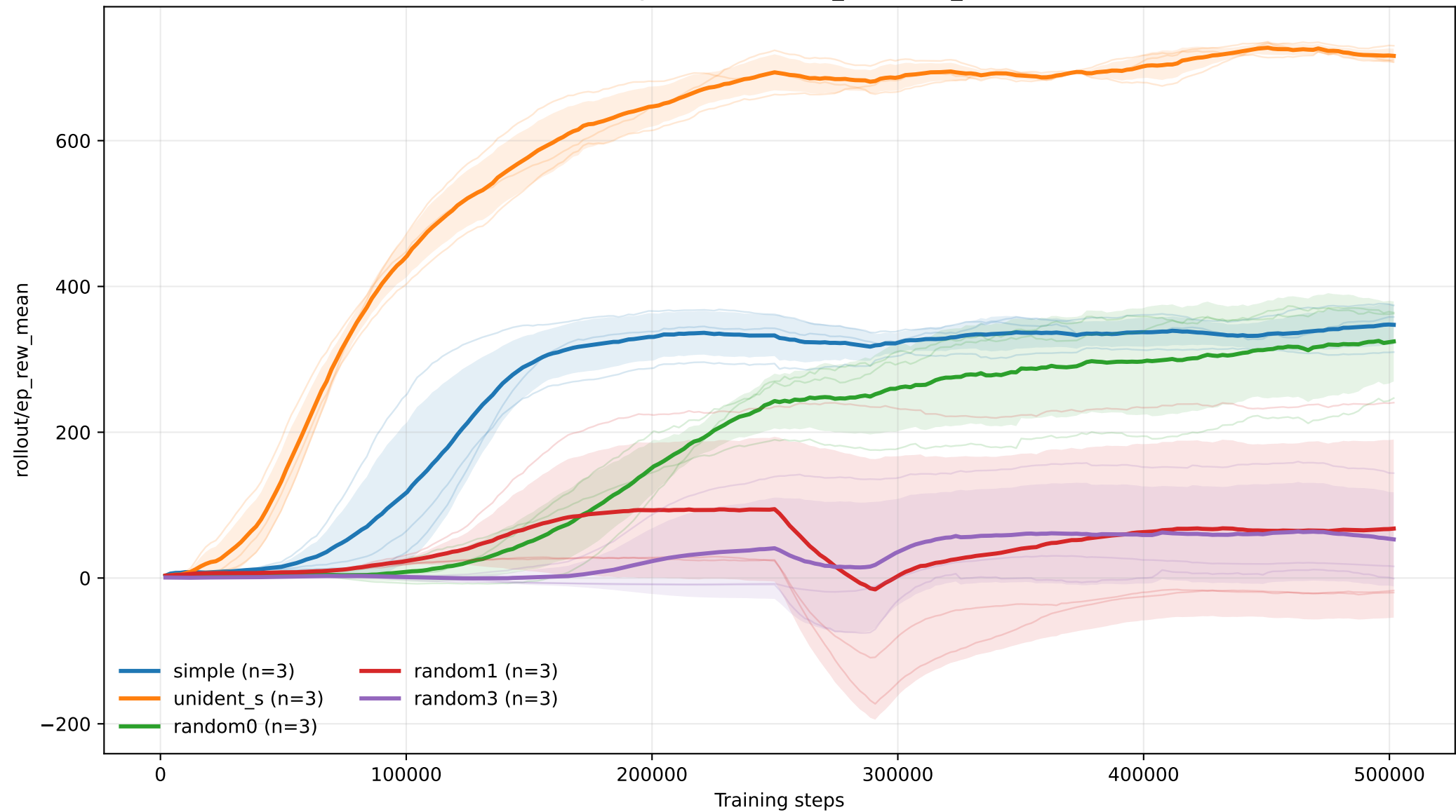
PPO training curves: v2extra_25 switch_250000
