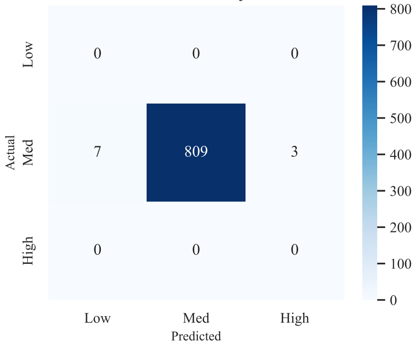
Confusion Matrix: Subject 1106
