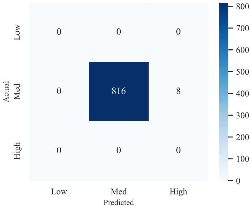
Confusion Matrix: Subject 1595
