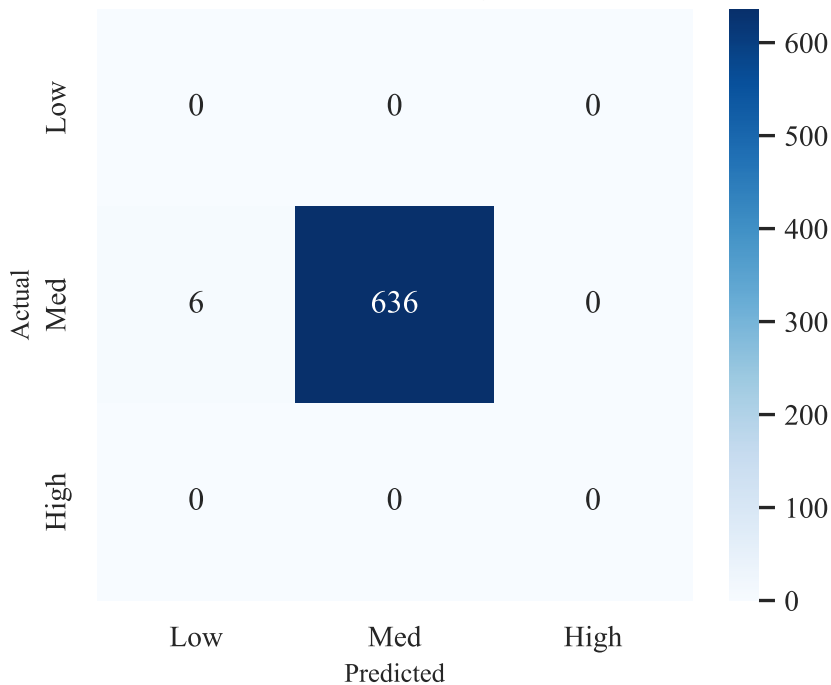
Confusion Matrix: Subject 1629
