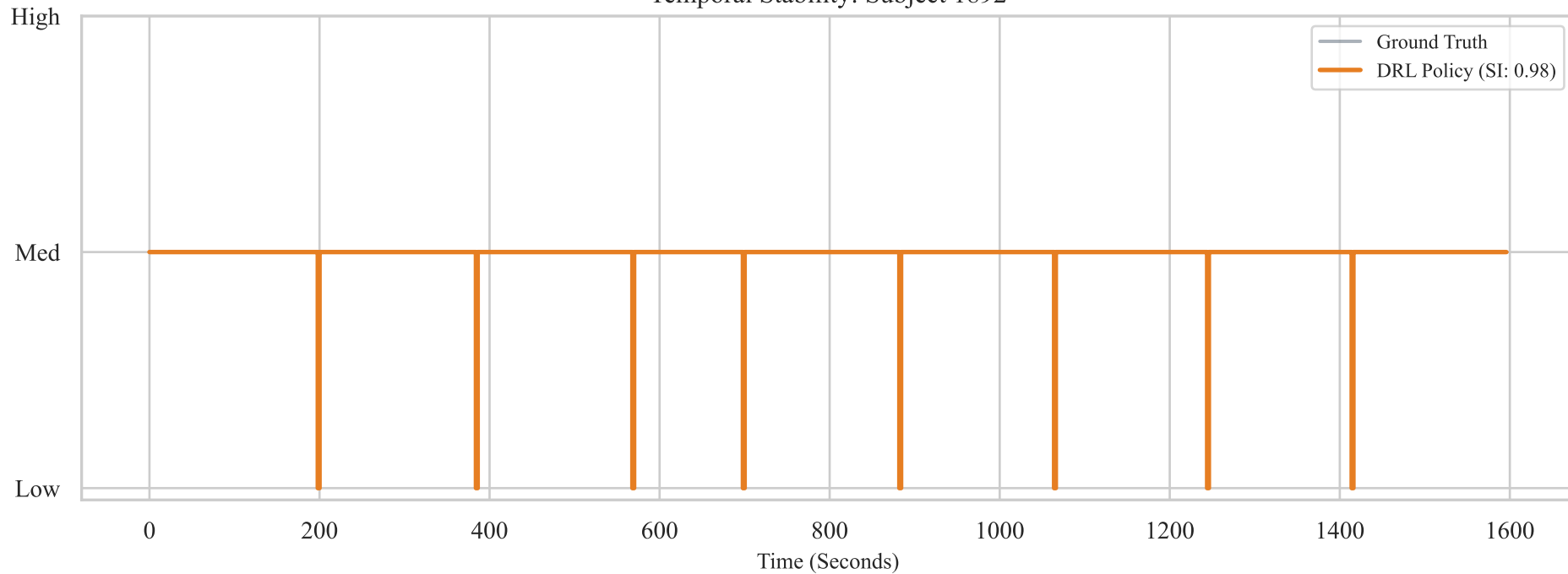
Temporal Stability: Subject 1892
