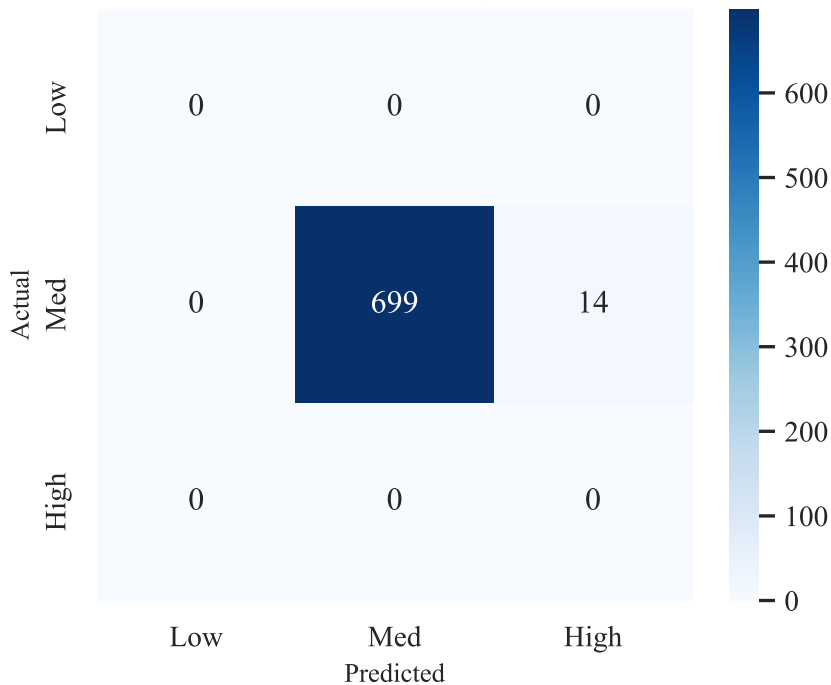
Confusion Matrix: Subject 1314
