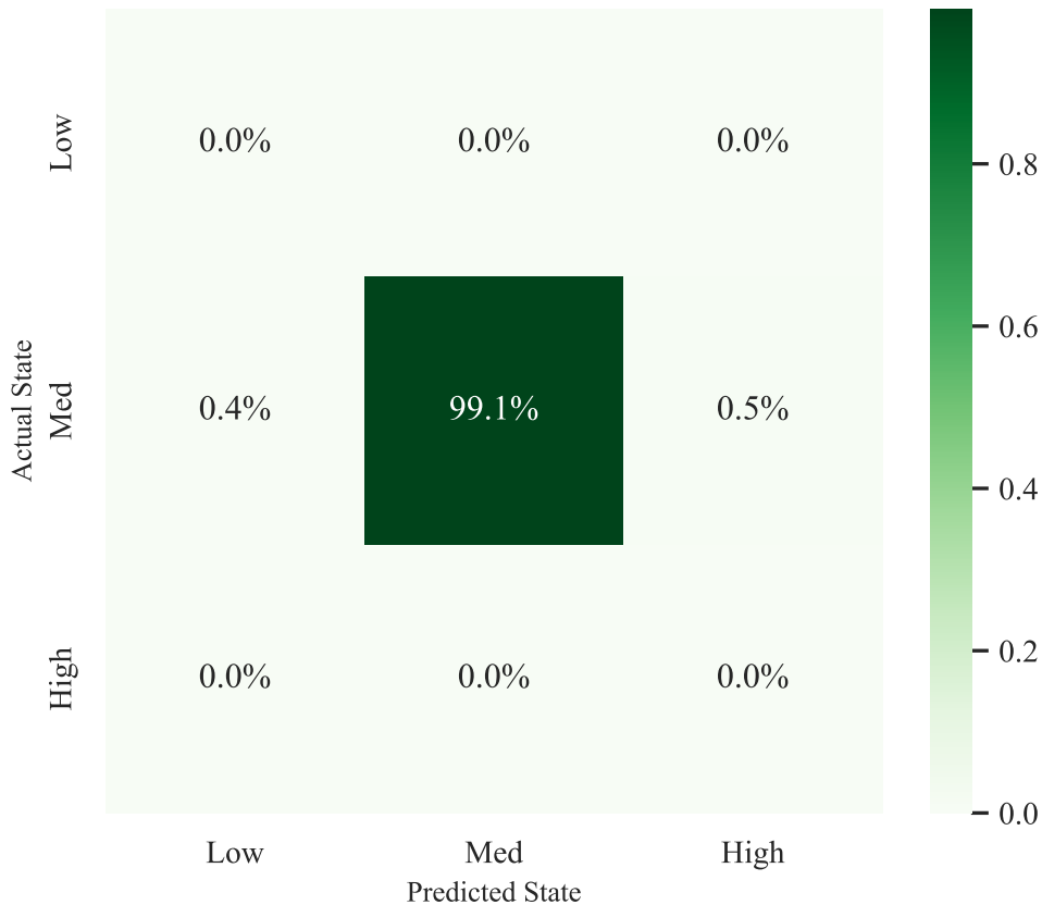
Normalized Global Confusion Matrix
