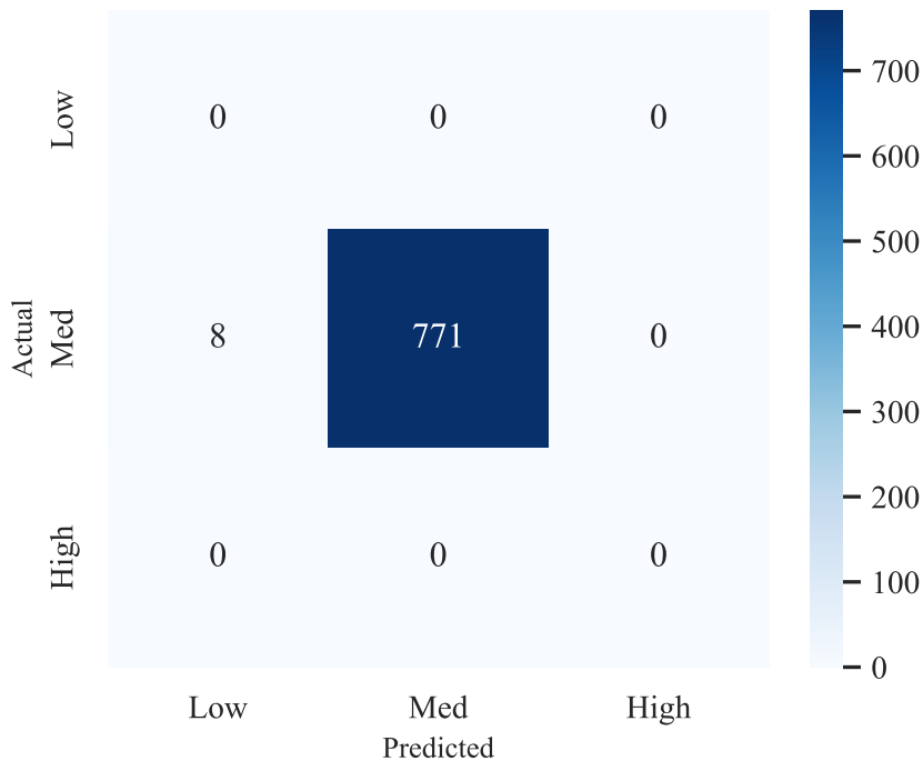
Confusion Matrix: Subject 1434
