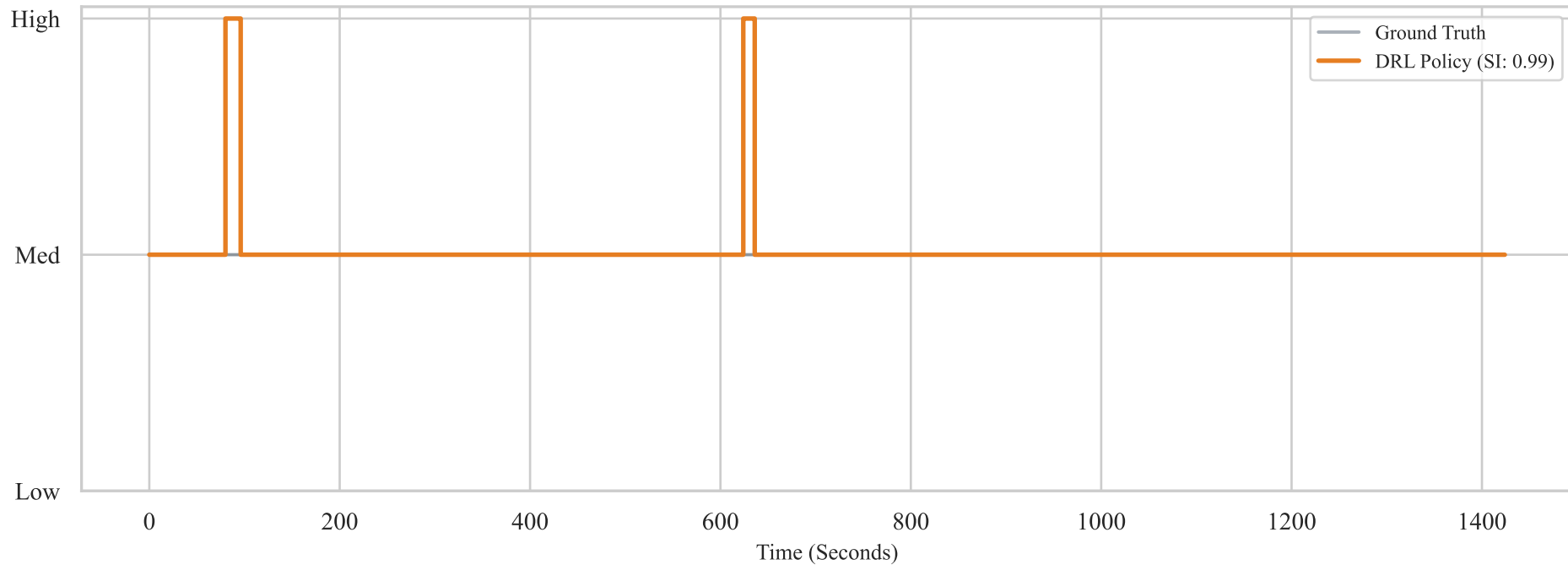
Temporal Stability: Subject 1314
