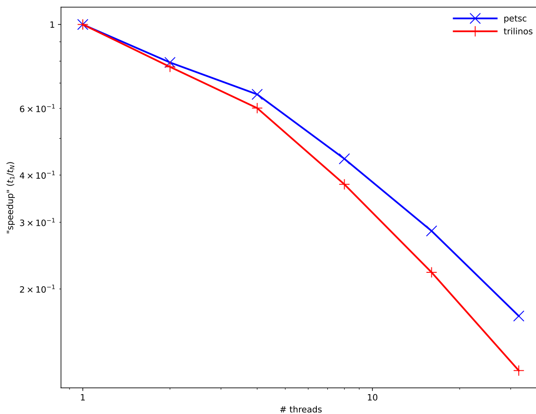
Fig. 1: Effect of having more OpenMP threads for each MPI rank Page 20, 1 .
