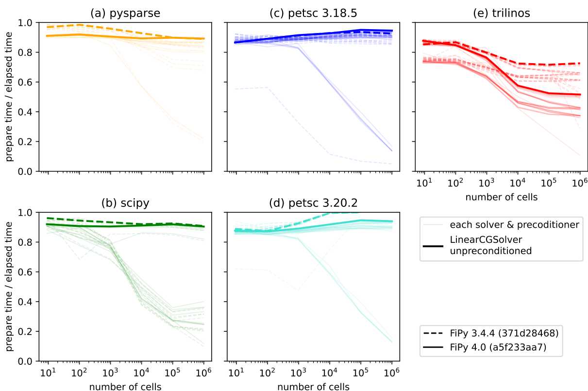
Fig. 2: Ratio of time to prepare the matrix to the combined time to prepare and solve the matrix for different solver suites, solvers and preconditioners, and different versions of FiPy Page 33, 4Page 33, 5 . The thick lines highlight LinearCGSolver with no preconditioner, one of the better-performing combinations available in all suites.
