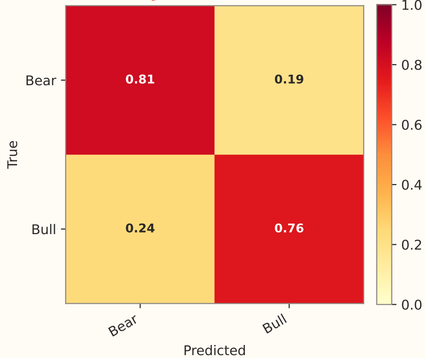
FinJEPA (F1=0.784)
