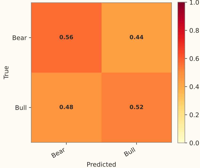
PatchTST (F1=0.558)
