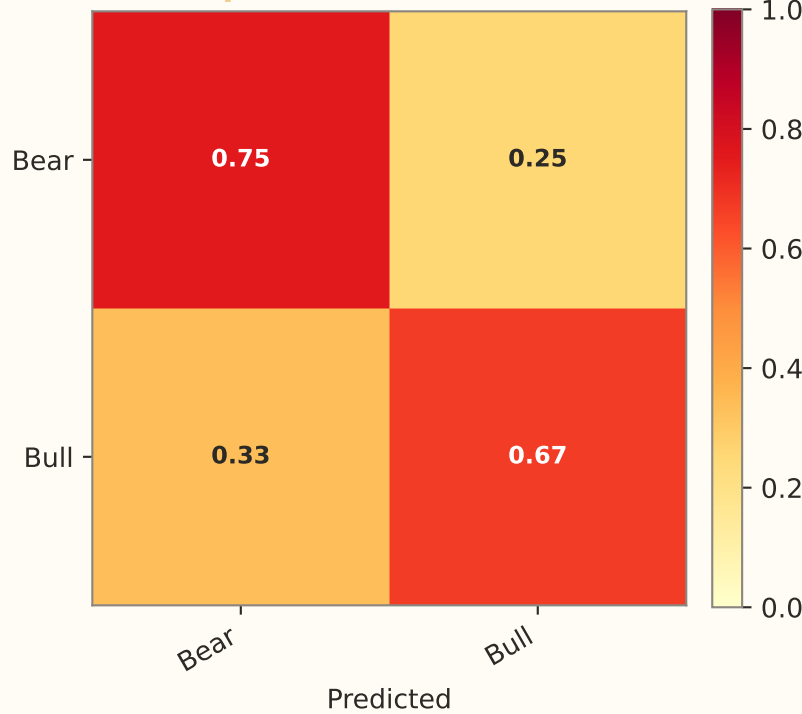
Supervised (F1=0.712)
