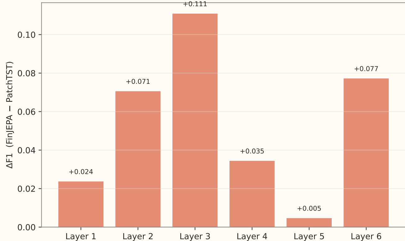
FinJEPA Advantage over PatchTST per Layer
