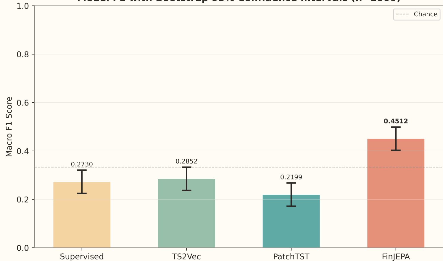
Model F1 with Bootstrap 95% Confidence Intervals (n=1000)
