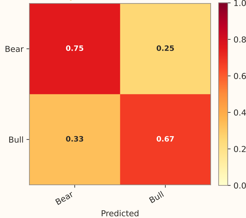
Supervised (F1=0.500)
