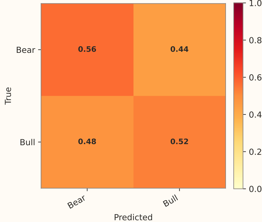
PatchTST (F1=0.621)
