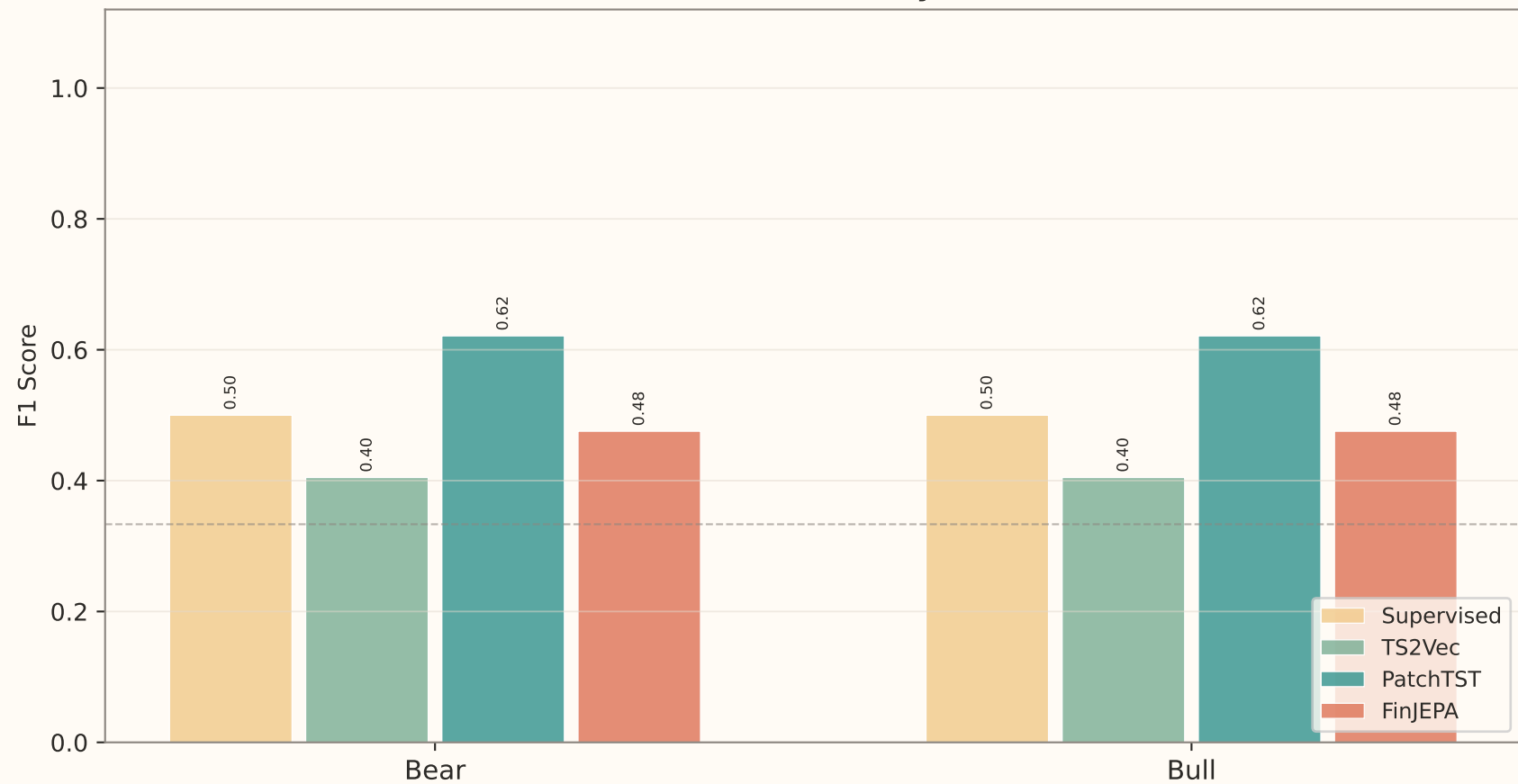
Per-Class F1 Score by Model
