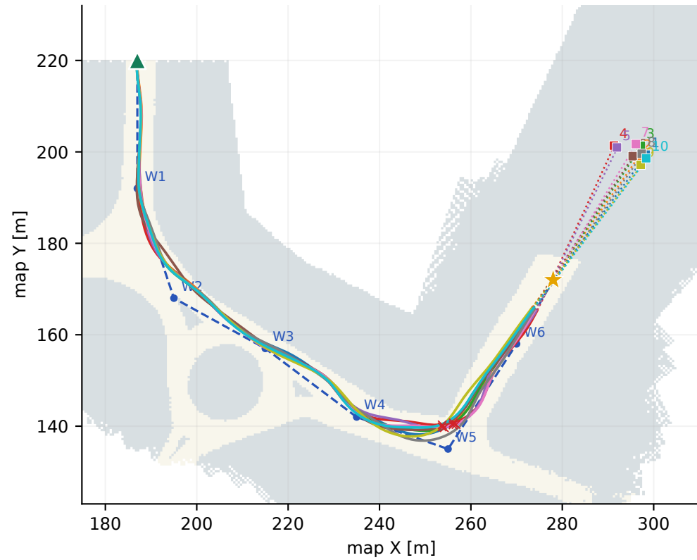
Scenario 3: 10/10 goal approaches 20261008_185426_scenario3_72c4df
