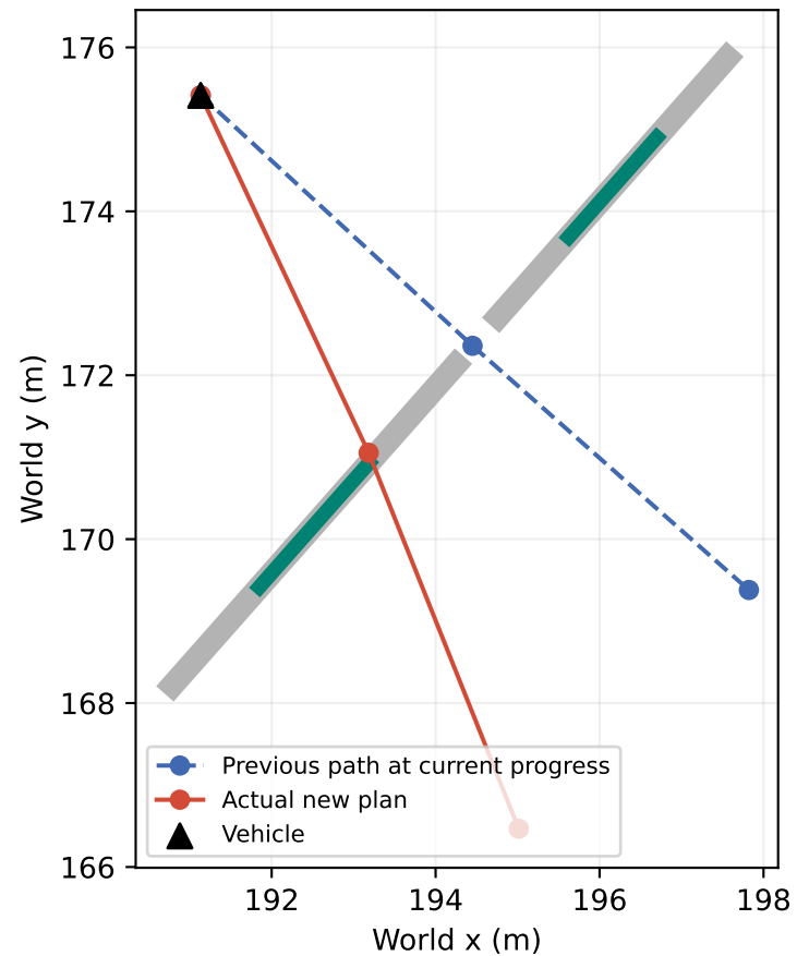
Actual S1 trace, 01:41:55 KST Gray: raw section; green: allowed section
