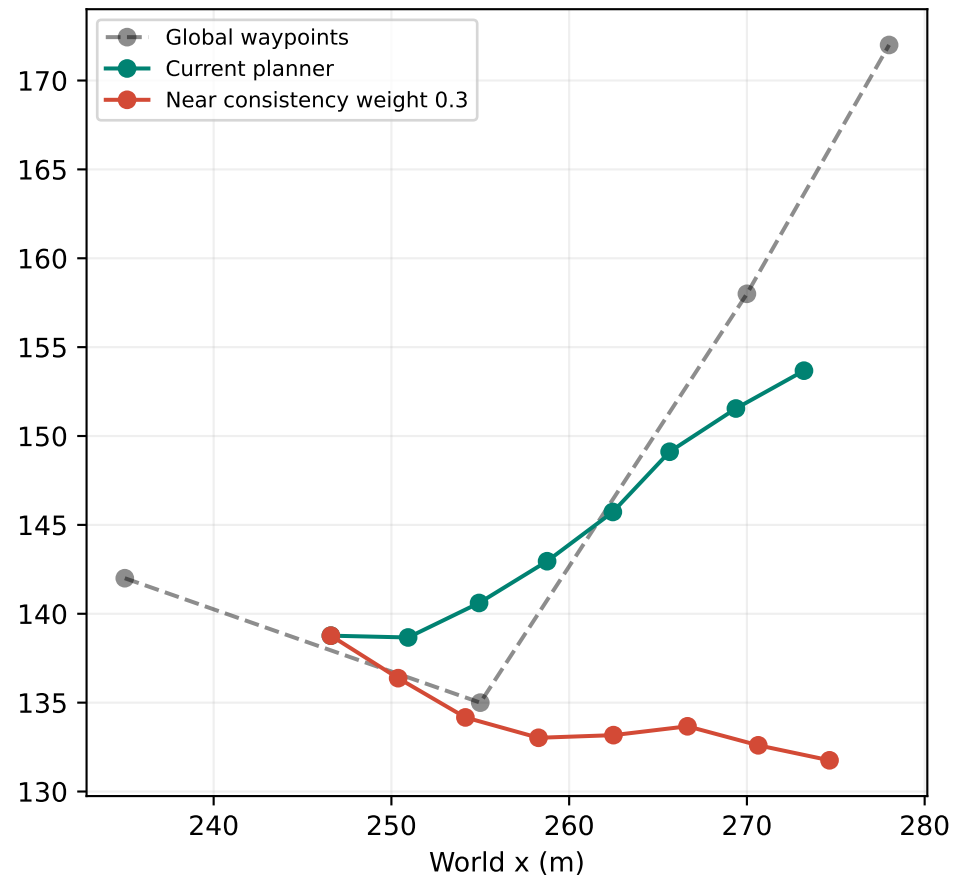
S2 fixed-pose replay, 01:43:24 KST Added cost keeps plan on the wrong arm
