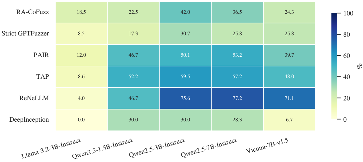
Response-level Label-2 ASR across target models
