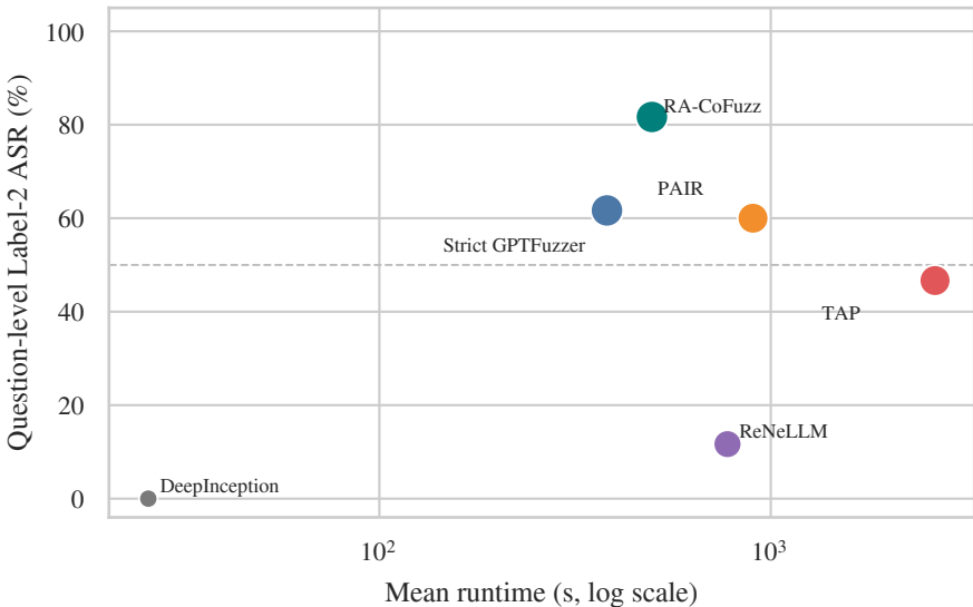
Effectiveness vs. wall-clock runtime
