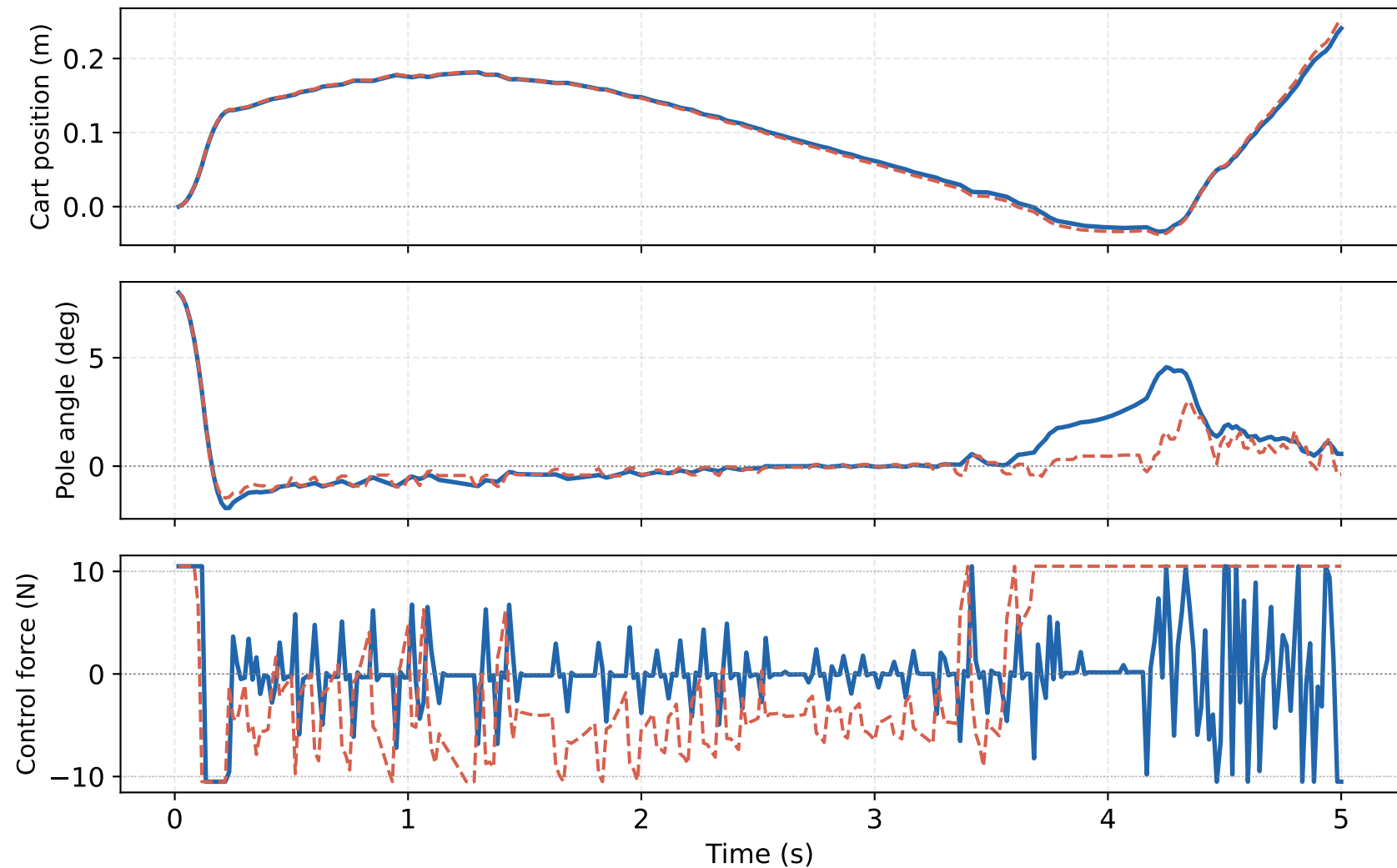
Cartpole Time Histories — Student Rollout, \theta_0 = 8^\circ
